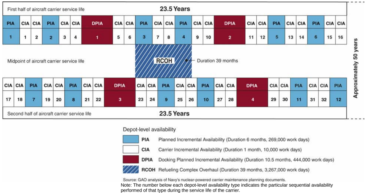
Figure 1: Depot-level Availability Maintenance Schedule of a Nuclear-Powered Aircraft Carrier over Its Expected 50-Year Service Life
