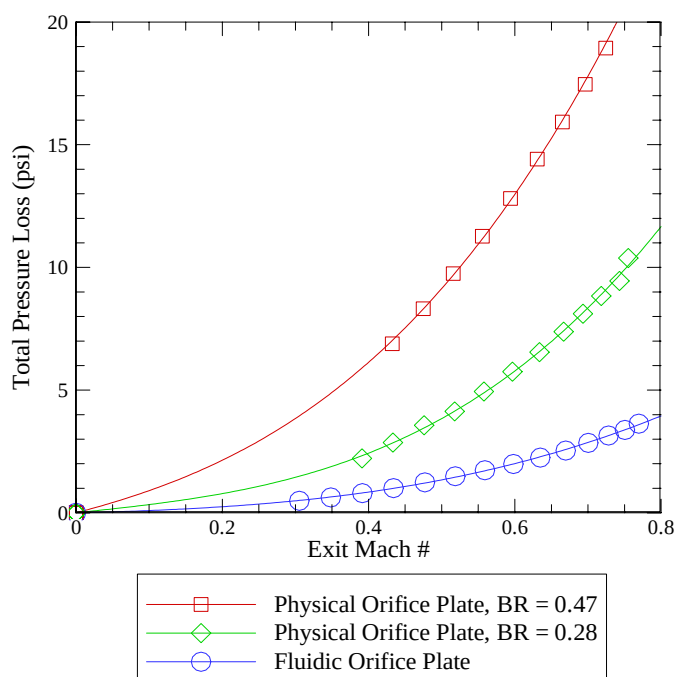
4 Draco Drive Figure 8. Estimated total pressure losses for different obstacle configurations j1) 275-5724
