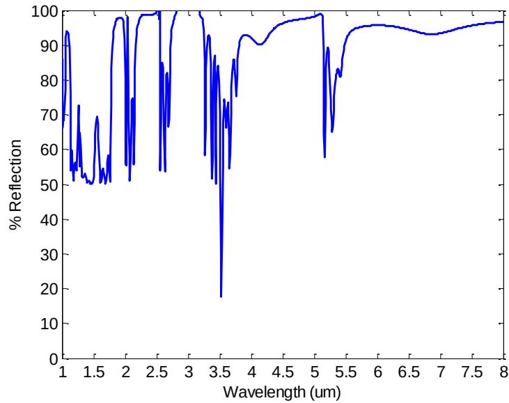
Figure 63 Plot of the reflection from the Au-SU-8 structure treated as a layered material at 61.3°. Note that there are points at 1.25um, 2.5um, and 3um where the reflection goes above 100%. This is due to total internal reflection that occurs from 1µm to 3.55µm.
