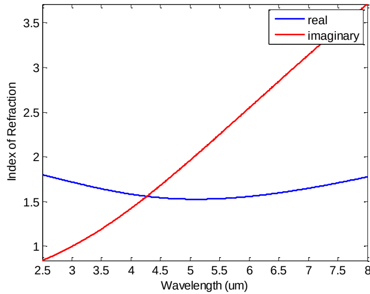
Figure 35 Plots of the effective index for Ti- \text{Al}_2\text{O}_3 structure derived from the effective permittivity.
