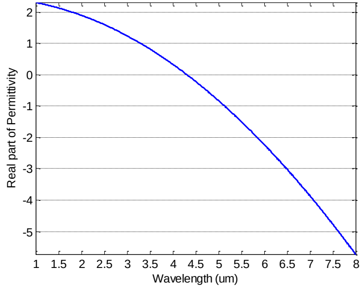
Figure 61 Revised plot of the effective permittivity of the Au-SU-8 structure with 4\mu\text{m} thick SU-8 layers, showing the shifted zero point.
