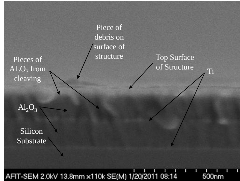
Figure 36 Micrograph of Ti- \text{Al}_2\text{O}_3 structure, showing the layers and the substrate. Notice that there is some debris on the layers since the \text{Al}_2\text{O}_3 did not cleave cleanly.
