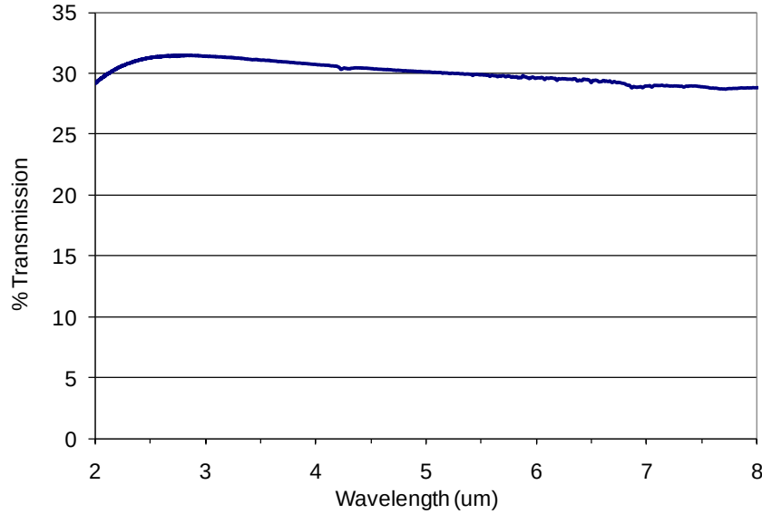
Figure 42 Plot of the FTIR transmission data for the Ti- \text{Al}_2\text{O}_3 structure at 0^\circ . The maximum is 31% at 2.76\mu\text{m} .
