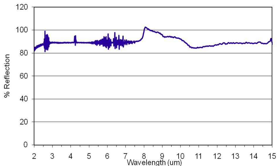
Figure 17 Reflectance measurement of Ag- Al 2 O 3 structure in the infrared at an angle of 61.3°. Notice that there is a peak that goes beyond 100% at 8µm and is not reliable data, likely due to a calibration error.
