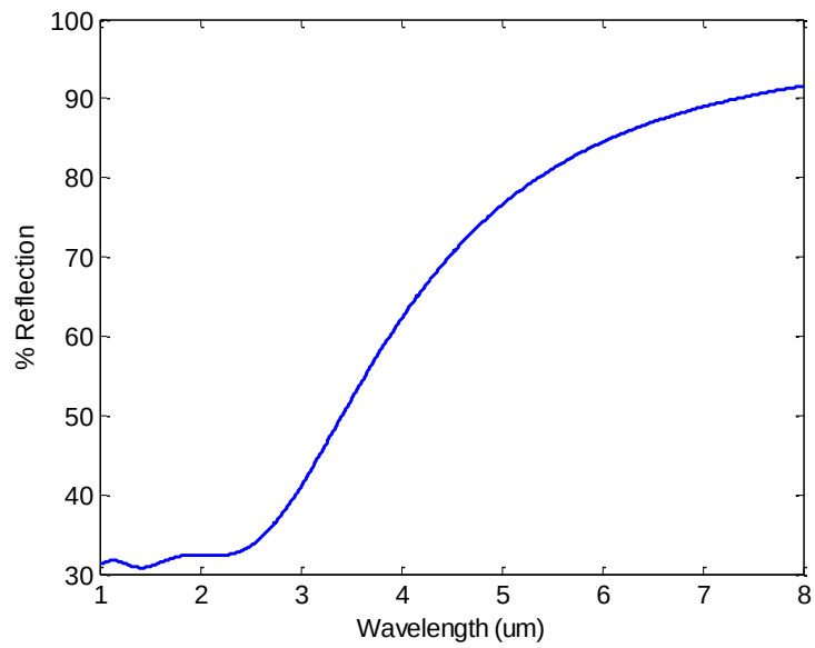
Figure 78 Plot of reflection from Ni-Si structure modeled as homogenous at 61.3°.
