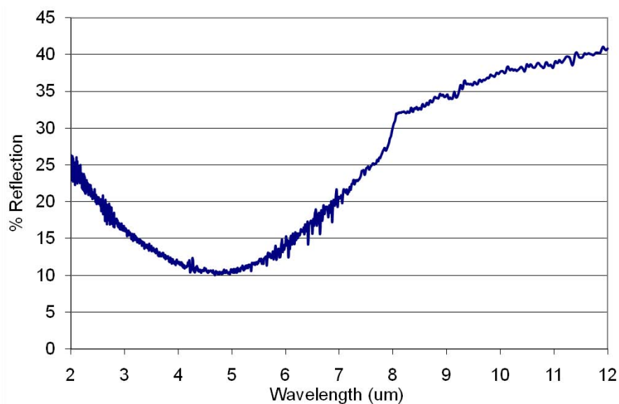
Figure 80 Plot of FTIR data for reflection from the Ni-Si structure. The noise towards 2μm is a result of the data being collected at the edge of the instrument's range.
