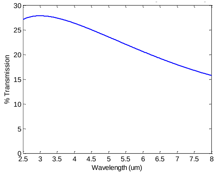
Figure 40 Plot of Transmission from Ti- \text{Al}_2\text{O}_3 Structure treated as homogeneous at 0^\circ .
