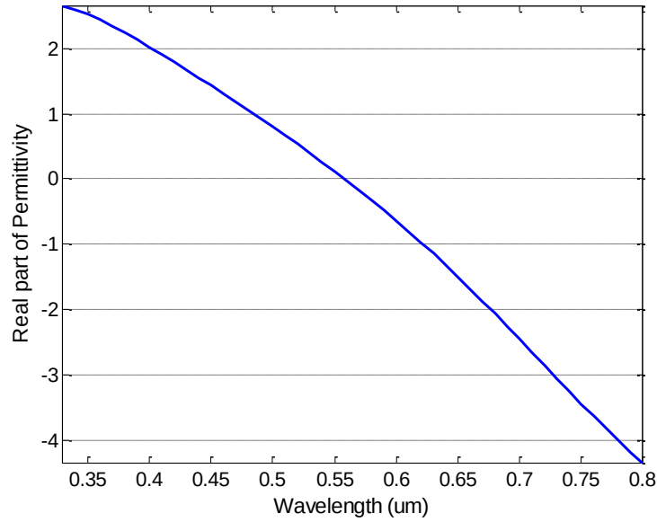
Figure 29 Plot of the effective permittivity of the one period Ag- \text{Al}_2\text{O}_3 structure on glass using the permittivity for the materials derived from the measured indices.
