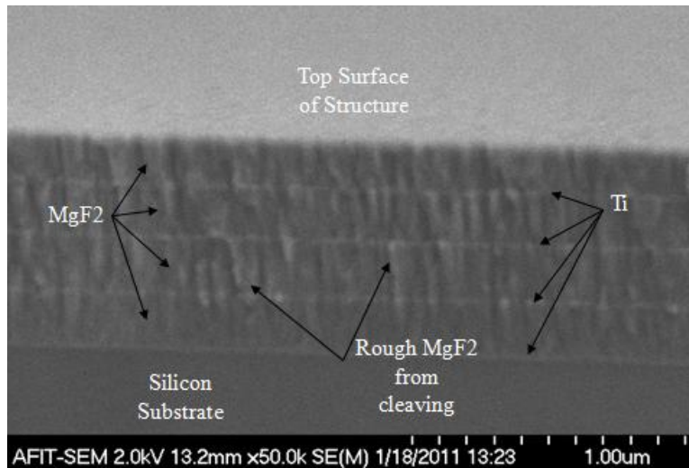
Figure 47 Micrograph of the fabricated \text{MgF}_2 structure. Note the thickness of the \text{MgF}_2 layers is approximately 155nm.
