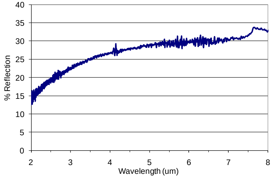
Figure 41 Plot of the FTIR reflection data for the \text{Ti-Al}_2\text{O}_3 structure at 61.3^\circ .
