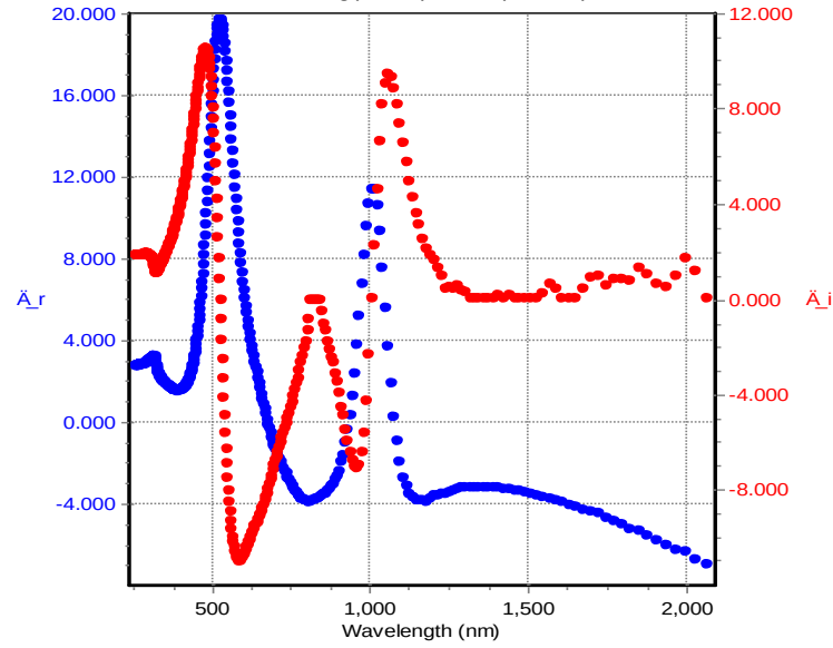
Figure 18 Calculated permittivity of the Ag-Al 2 O 3 structure as homogeneous using ellipsometry. The blue points and left axis are for the real part of the permittivity, and the red points and right axis display the imaginary parts. Note that the plots are a function of wavelength in nm.
