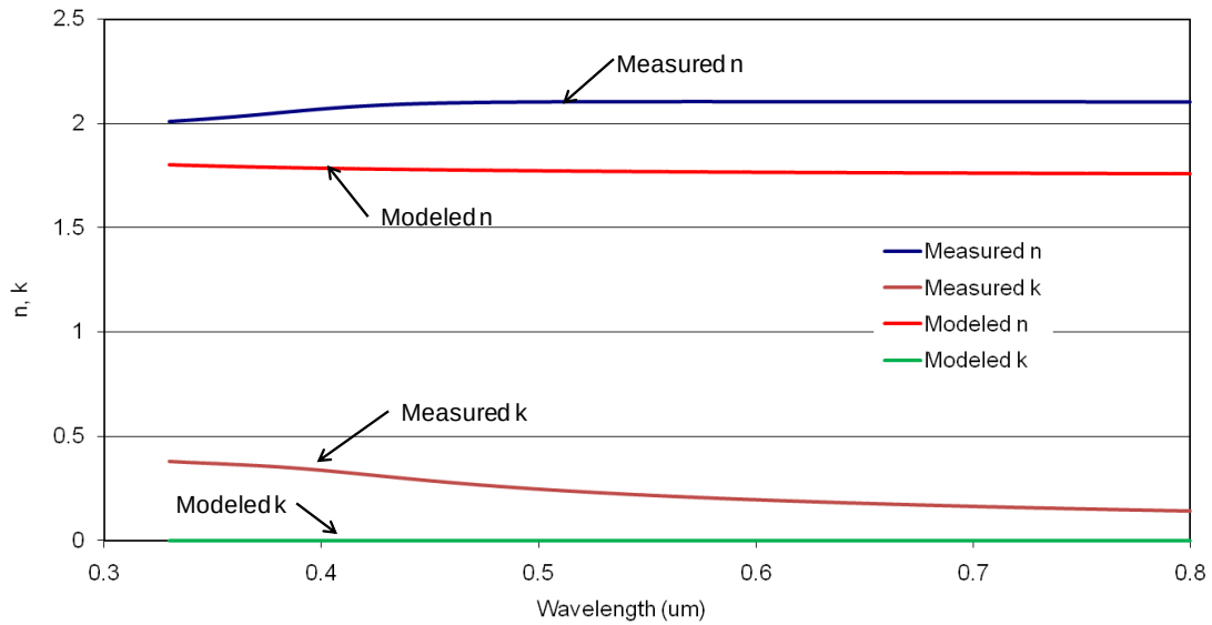
Figure 28 Plot of the modeled and measured index of \text{Al}_2\text{O}_3 deposited on glass.
