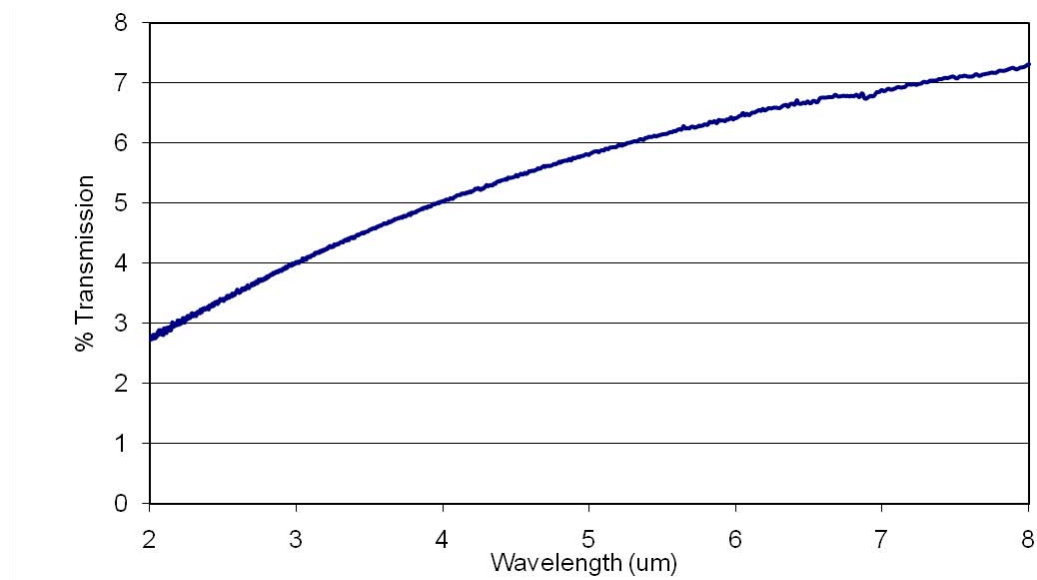
Figure 55 Plot of transmission data from the Ti- \text{MgF}_2 structure at 0^\circ .
