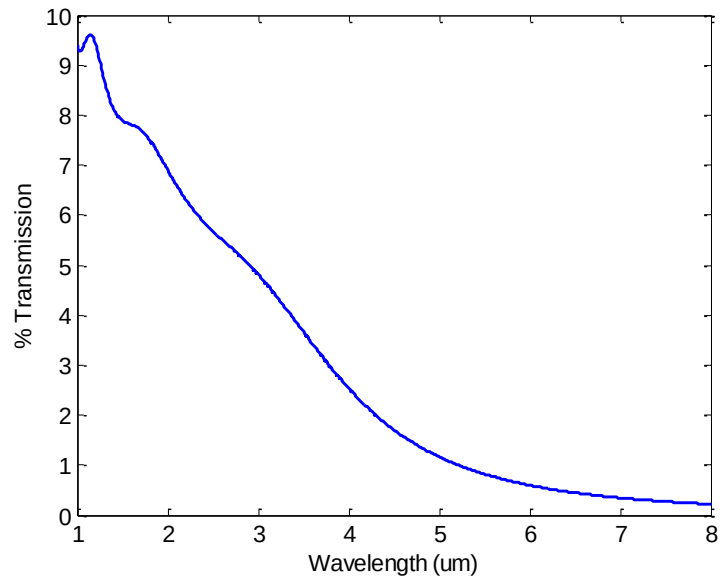
Figure 77 Transmission from Ni-Si structure modeled as layered media at an incident angle of 0°.
