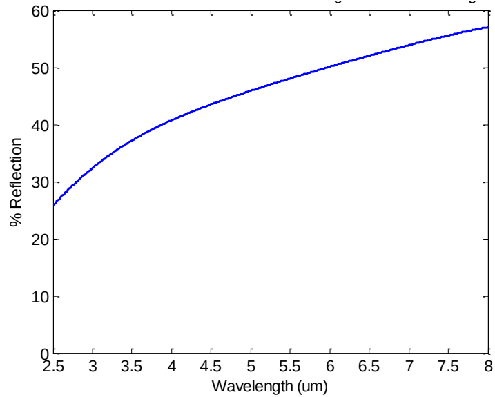
Figure 39 Plot of reflection from Ti- \text{Al}_2\text{O}_3 structure modeled as homogeneous at 61.3^\circ .
