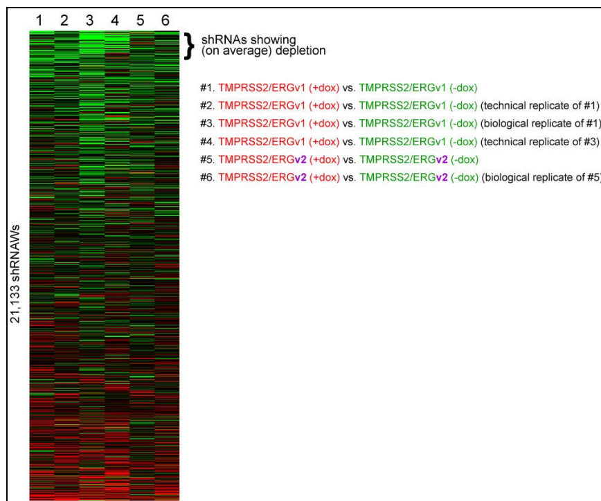
Fig 3. Whole-genome shRNA screens. Heatmap summarizes results of whole-genome (21,000) shRNA screens of RWPE1-TMPRSS2/ERG variant 1 (v1) and variant 2 (v2). Each of the six columns is a separate screen/microarray. Each row is a different shRNA, ordered by magnitude of average depletion (green) and enrichment (red). shRNAs exhibiting, on average, depletion are bracketed.
