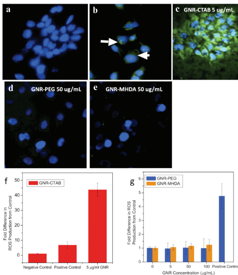
Figure 3. Oxidative stress production after exposure to GNR-CTAB. (a) Negative control; (b) positive control (0.03% \text{H}_2\text{O}_2 ); (c) 5 \mu\text{g}/\text{mL} GNR-CTAB, (d) 50 \mu\text{g}/\text{mL} GNR-PEG, (e) 50 \mu\text{g}/\text{mL} GNR-MHDA. Nuclei are stained with Hoechst, and the DCFH probe fluoresces green in the presence of ROS. White arrows indicate green fluorescence produced in positive control. (f) Oxidative stress production after exposure to GNR-CTAB and (g) GNR-MHDA and GNR-PEG. Data were normalized FITC intensity to Hoechst intensity to account for cell number.
