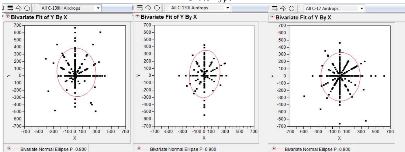
Figure 4.4: All Data Scatterplots by Aircraft Type
