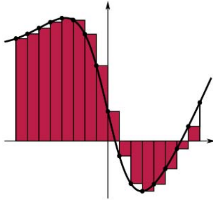
Figure 4.12: Rectangular Method Numerical Integration (KSmrq, 2011)
