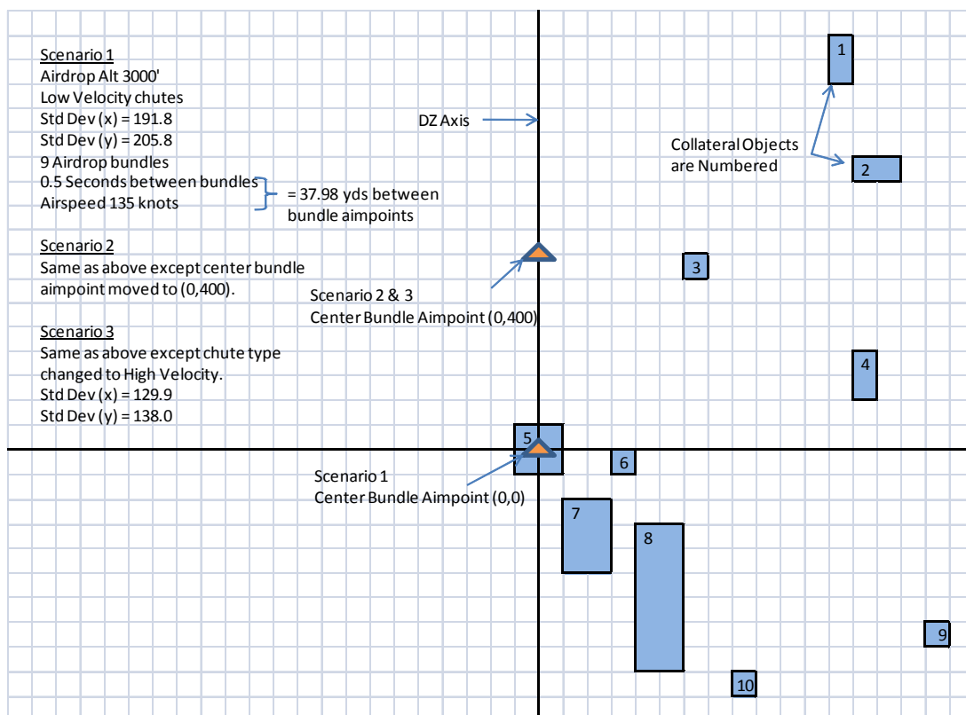
Figure 4.17: Graphic Example of Risk Estimation Scenarios
