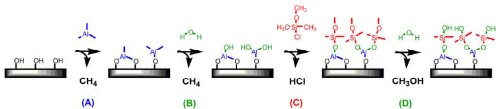
Figure 9 Schematic showing the four-step reaction sequence for ABCD MLD growth of an alumina-siloxane film using trimethylaluminum (TMA), H 2 O, dimethylmethoxychlorosilane (DMMCS) and H 2 O.
