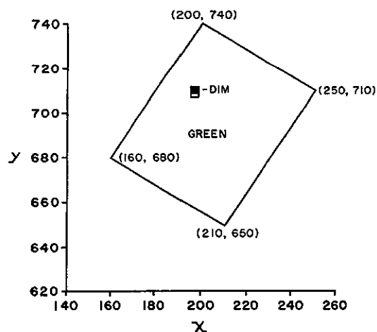
Figure 4. CIE (1931) chromaticity specification limits and plots for Green and Dimmed Green filters.
