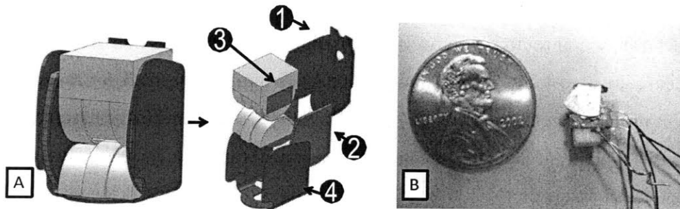
Figure 1.1: Sample solder-activated joint. (A) The joint, in light grey, uses flexures to keep the top and bottom half-cylinders in contact. Rolling of the top half-cylinder over the bottom is constrained when the solder (2) between the two copper pieces (1 & 4) is solidified. Current is run through a strain gage (3) within the joint to melt the solder. (B) Picture of an actual solder activated joint designed and built using this thesis.
