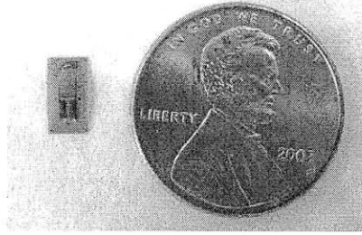
Figure 3.13: Vishay 062AK EA series strain gage. This strain gage was used as the heater mechanism in Squishbot1.
