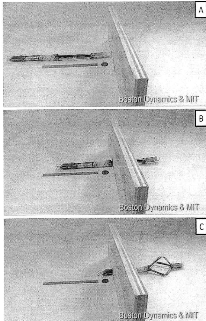
Figure 4.25: Squishbot1 traversing a 20mm hole. In A &B, all the joints are locked in the extended leg position, and a prismatic joint is used to advance the mechanism. In C, the joints have been unlocked and the robot begins to crawl using the tripod structure.
