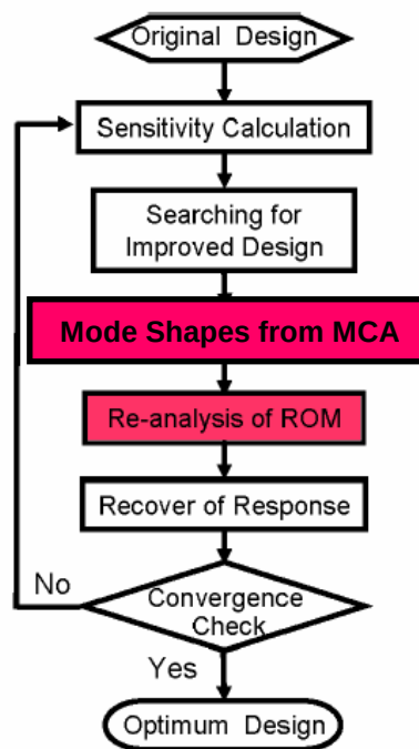
Figure 1. Flowchart for MCA-enhanced NASTRAN optimization
