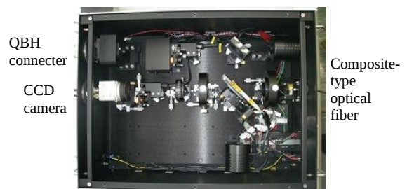
Fig. 6 Inside view of the coupling device housing
