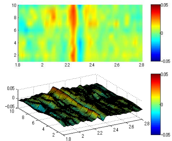
Fig. 8 ECT detection for a crack on a 1 inch diameter tube (a) noise filtered signal, (b) stereoscopic view
