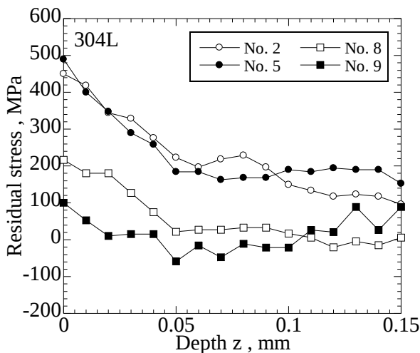
Fig. 7 Distribution of residual stress
