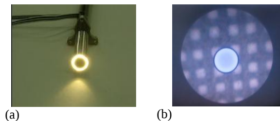
Fig. 3 Composite-type optical fiber (a) telescope section, (b) image view of 0.15 mm mesh
