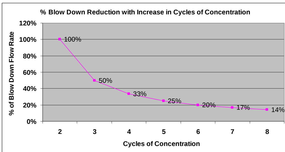
Figure 4: Percentage blow-down reduction with increase in cycles of concentration.
