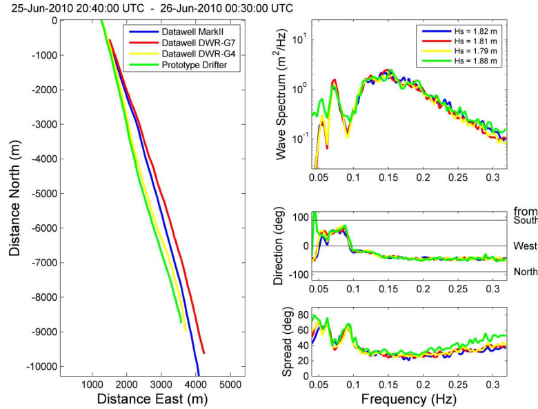
Figure 6. Inter-comparison of free drifting Dataswell buoys (a 90 cm diameter accelerometer-based MKII and GPS-based 70 cm DWR-G7 and 40 cm DWR-G4) and our prototype GPS drifter during a 4-hour deployment when the buoys and drifter remained in close (less than 1.5 km) proximity of each other. Left panel: drift tracks. Right panels from top to bottom: surface height spectrum and mean direction and directional spread (as functions of frequency). Estimates of the significant wave height are listed in the legend of the upper right panel.
