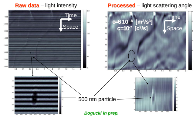
Figure 2. Raw (intensity) and processed (light scattering angle) images acquired for a controlled flow with a single 500 \mu\text{m} particle. The images were acquired over \sim 5 \text{ cm} aperture in 5 minutes.
