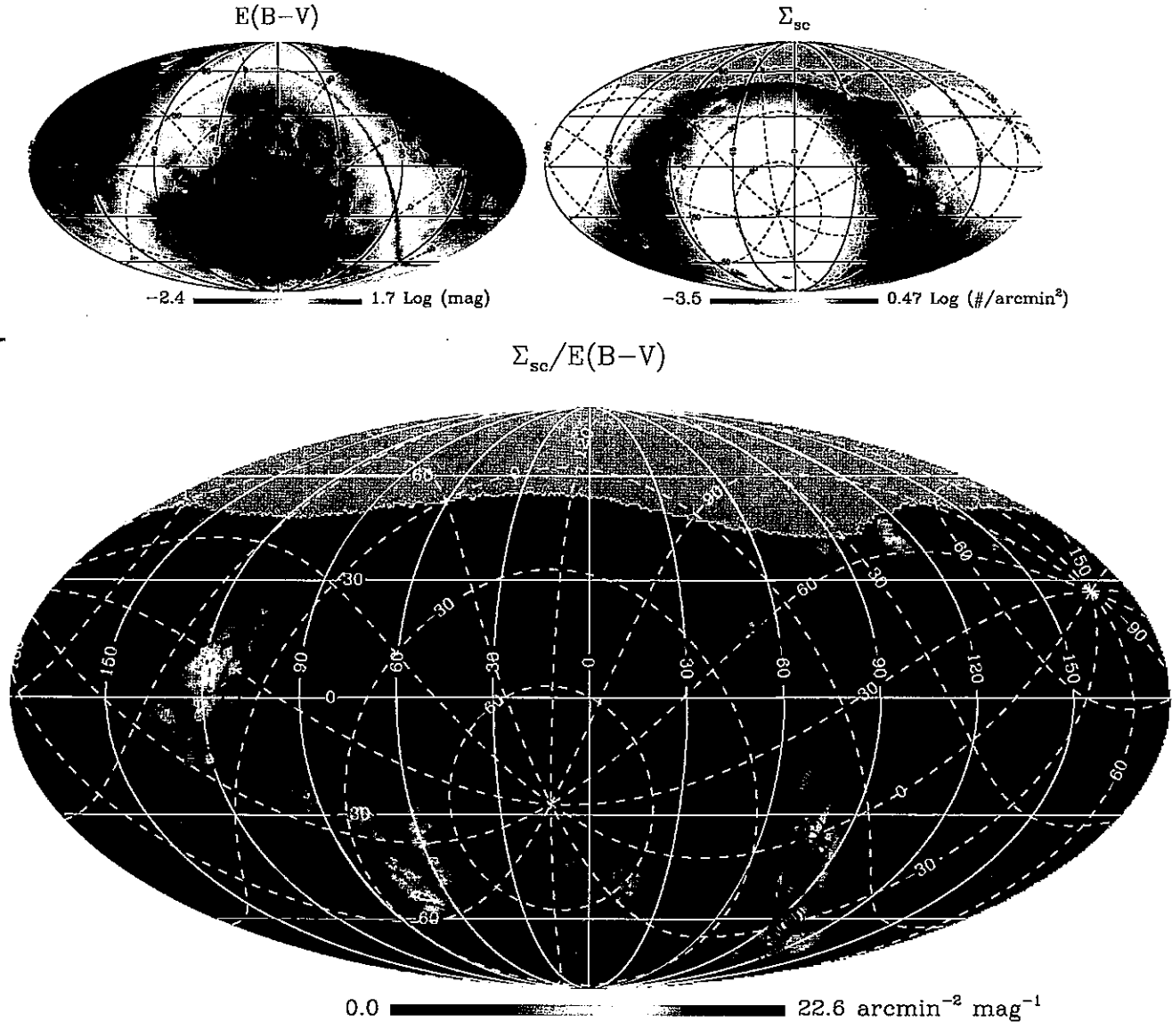
FIG. 3.— Top left : An all-sky map of extinction, scaled logarithmically. The solid-line grid corresponds to the celestial coordinate system with right ascension in degrees increasing to the left. Zero degrees lies at the center of the figure. A Galactic coordinate system is overplotted with dashed lines. Top right : The corresponding map of star-count surface density for stars in the 13–16.5 mag range. The region shown in gray corresponds to a high-declination gap in coverage in the UCAC2 stellar catalog. As noted in the text, any AO-friendly fields that might exist at very high declination would be unsuitable for other reasons. Bottom : A map constructed by multiplying the map at the top left by the inverse of the map at the top right. Maxima in this figure correspond to potentially interesting locations for undertaking extragalactic adaptive optics observations. Circles present the positions of 67 fields that are well suited to extragalactic AO. See the text for details. See the electronic edition of the PASP for a color version of this figure.
