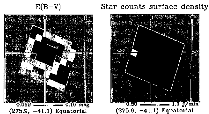
FIG. 11.—Extinction and star surface density maps of the 6.871'' \times 6.871'' cells within the 55' \times 55' field with the highest mean star-count surface density of \langle \Sigma_{sc} \rangle = 1.3 \text{ arcmin}^{-2} (i.e., with 11,000 star-forming galaxies potentially observable with AO if the average number surface density of these objects is 3 \text{ arcmin}^{-2} ). The field is centered at \alpha = 18^h 23^m 39.53^s and \delta = -41^\circ 6' 44.3'' . The solid-line grid corresponds to the celestial coordinate system with R.A. [\circ] = 360^\circ - \alpha [\circ] . See the electronic edition of the PASP for a color version of this figure.
