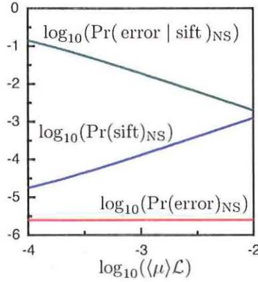
FIG. 3: (Color online) No-scintillation sift probability, error probability, and quantum bit-error rate plotted versus the logarithm of the average fractional power transfer, \langle \mu \rangle \mathcal{L} . These curves assume n_S = 0.5 , n_N = 5 \times 10^{-6} , and \eta = 0.5 .
