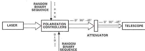
FIG. 1: Block diagram of a single-laser QKD transmitter (Alice). The laser output is a stream of linearly-polarized pulses. The polarization controllers are driven by a pair of random binary sequences. The first sequence determines the sequence of polarization bases that will be sent: + = 0^\circ/90^\circ or \times = \mp 45^\circ . The second sequence determines the bit value to be sent, according to the coding rule given in Eq. (1). The attenuator reduces the transmitter's output to n_S photons, on average, per bit interval.
