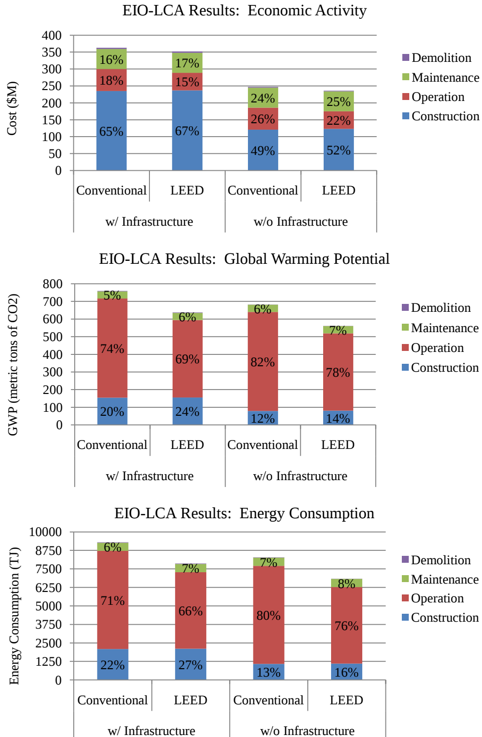
Figure 2. LCA results, with and without support infrastructure, comparison of total economic activity, environmental impact and energy consumption
