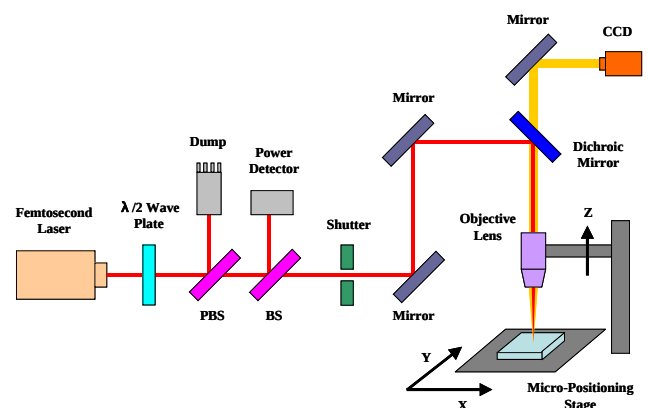
Fig. 1 Schematic illustration of the femtosecond laser system.
