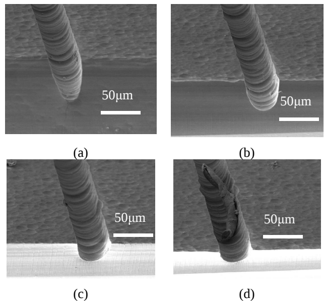
Fig. 4 SEM images of irradiated Foturan glass after heat treatment and etching: (a) 0.23 mW, (b) 0.27 mW, (c) 0.30 mW, and (d) 0.33 mW.
