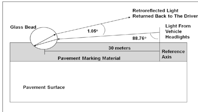
Figure 1-1: Retroreflectivity Illustration
