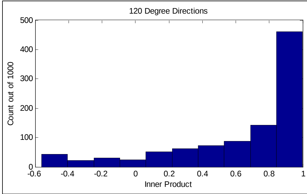
Figure 4. Inner products for 120° separation of directions.
