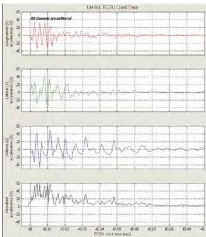
Figure 6 Unfiltered acceleration time-history traces from Electronic Crash Sensor Unit (ECSU)
