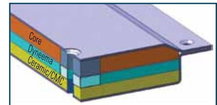
Figure 7 Typical IAF Section Cut
