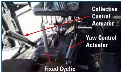
Figure 3 Collective, Cyclic and Yaw Control
