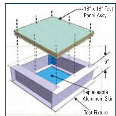
Figure 8 IAF Test Panel Configuration
