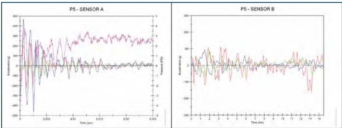
Figure 7 Helmet acceleration time-history data traces from the internal and external Helmet Sensor (HS) systems
