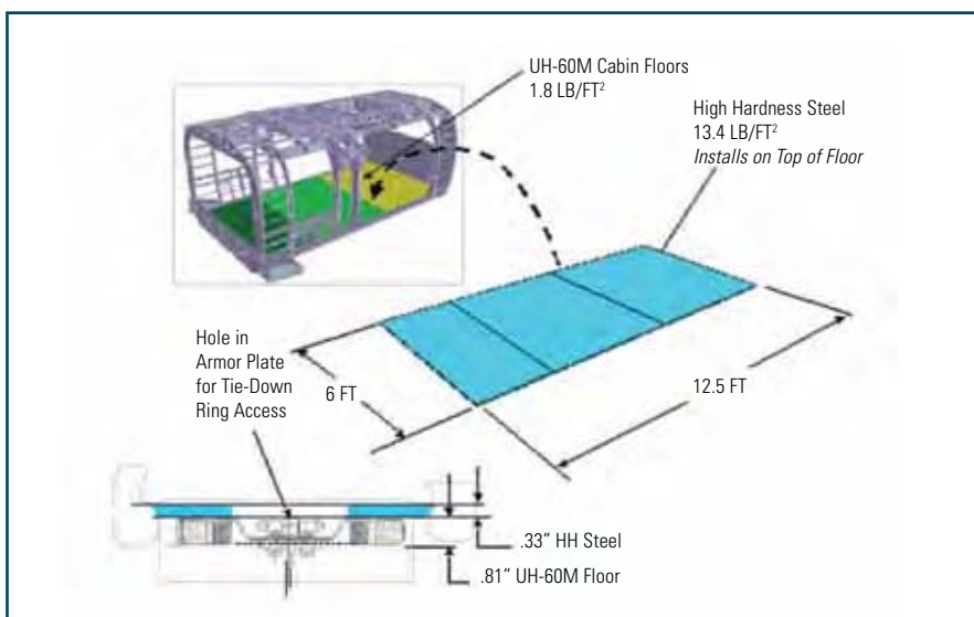
Figure 1 Baseline Floor/Armor System in UH-60 Cabin
