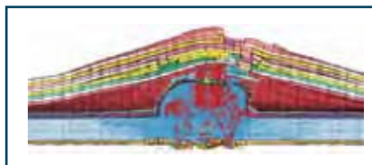
Figure 4 Mixed Lagrangian and SPH Simulation of the Bullet Impacting the Floor Section
