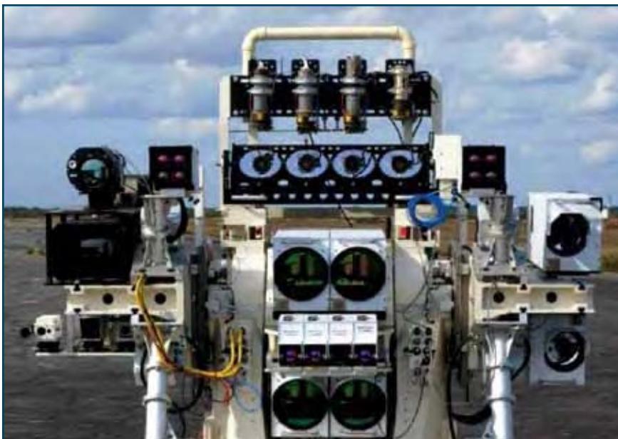
Figure 3 JMITS Missile Plume Simulator with captive seekers
