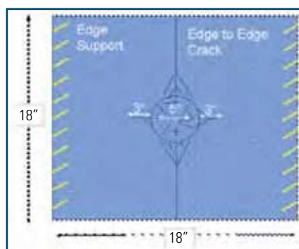
Figure 11 Ceramic/CMC Crack Pattern Post Box Drop
