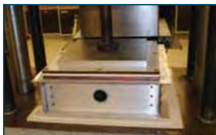
Figure 9 Sub-Element in Load Frame
