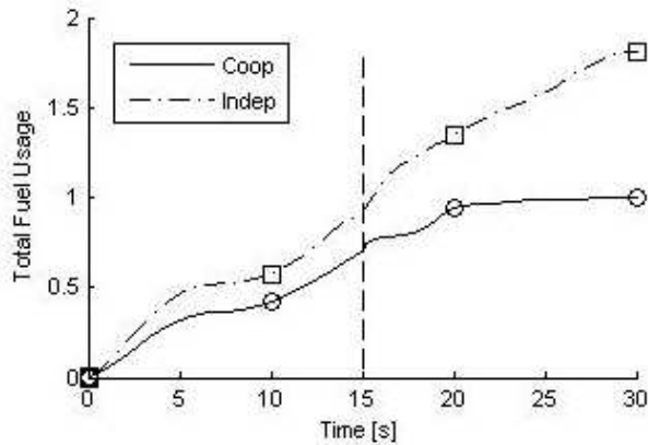
Fig. 4. Simulation total fuel consumption. The vertical line indicates the switch from translation to rotation
