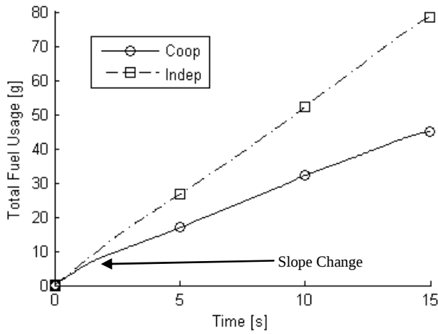
Fig. 6. Median fuel consumption for Cooperative and Independent Control. Note the distinctive reduction in slope of the Cooperative line at time 1.5 s.
