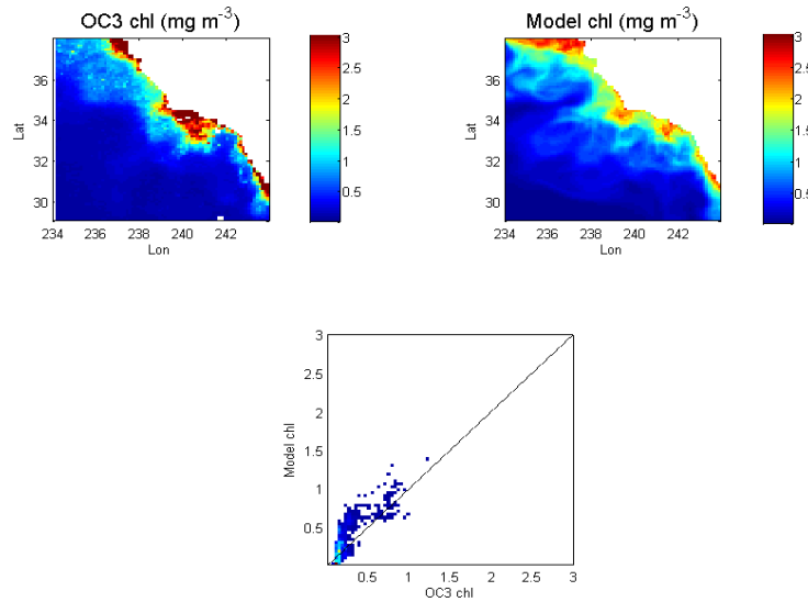
Figure 3: Spring (Mar, Apr, May 2006) averaged comparison between the modeled (12.5 km resolution) and satellite derived chlorophyll concentration. The model results are from 12.5 km high resolution Pacific ROMS-CoSiNE model.
