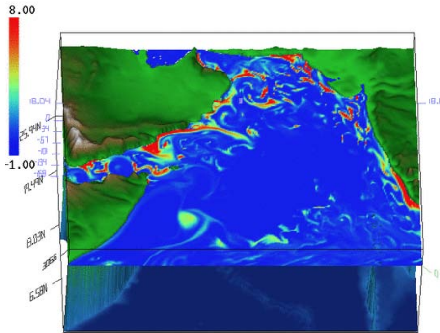
Figure 4: A snapshot of the modeled surface chlorophyll in mid July. The NCOM-CoSiNE clearly shows the upwelling signature along the coast of Oman, which in response to the Southwest Monsoon. The diatom is the dominated phytoplankton species along the coastal region. The modeled surface chlorophyll tends to match with the remote sensing observations very closely.
