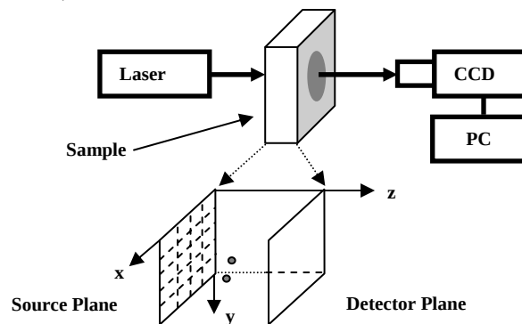
Fig. 1. A schematic diagram of the experimental arrangement used for imaging objects embedded in a turbid medium. Inset shows the 2D array in the input plane that was scanned across the incident laser beam.
