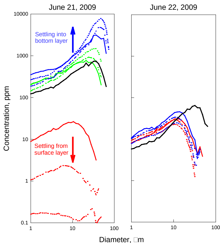
Figure 5: Disaggregated inorganic grain size distributions for samples collected at 30 cm below the surface (red), 10 cm above bottom (blue) and 50 cm above bottom (green) during maximum flood when flow speeds went from approximately -0.25 (solid line) to 0 (dashed line) to +0.25 \text{ cm s}^{-1} (dashed and dotted line). The black line is the size distribution of the suspension immediately after the passage of the tidal bore. The surface salinity range on June 21 was 14-19 and on June 22 was <1. Data for the 50 cm above bottom samples on June 22 were omitted for clarity but were the same as those for 10 cm above bottom.
