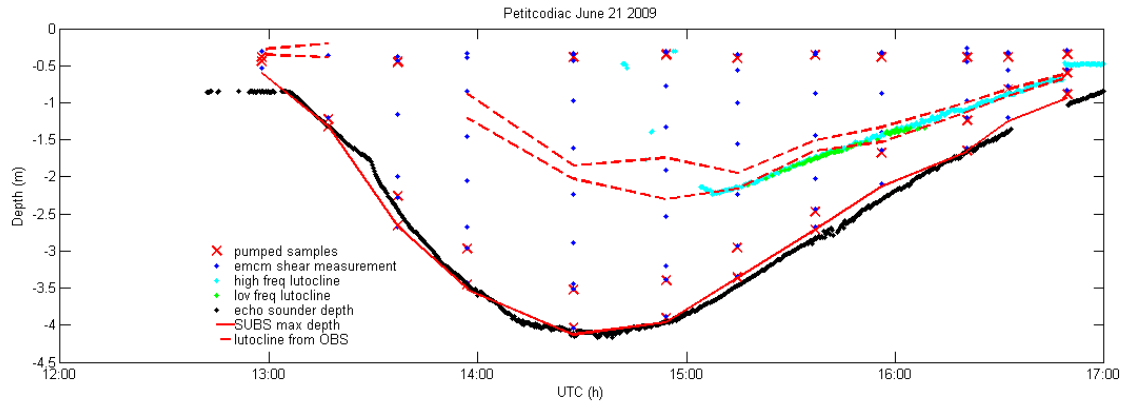
Figure 3: Summary of sampling from the SUBSI profiler and Knudsen dual frequency echo sounder mounted on a surfboard 10 m away. The close comparison of water depth from the two different instrument packages, as well as good agreement in the depth to the lutocline using acoustic (dual frequency echo sounder) and optical (optical backscatterance) methods is encouraging for combining measurements from different instruments to obtain coverage over a range of conditions.
