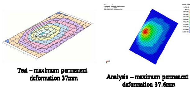
Figure 8 Comparison between test results and BEST simulation of the permanent deformation induced in one of the two sections of the outer V-shaped bottom structure
