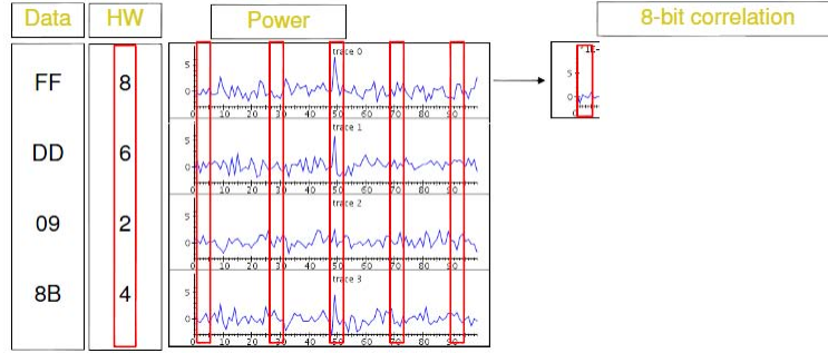
Figure 4. Correlation Power Analysis
