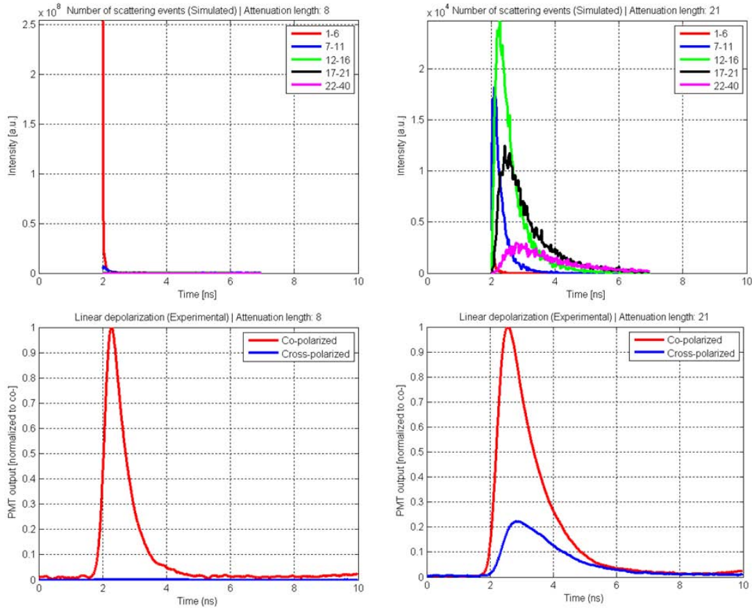
Figure 6: Time histories of both simulated (above) and measured (below) short pulses. The figure pair on the left shows the result from weakly scattering medium and on the right from significantly more turbid medium (magnesium hydroxide).
