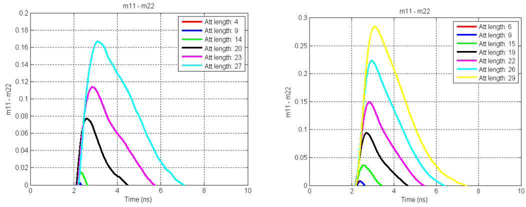
Figure 7: Mueller Matrix elements m_{11} - m_{22} of the measured pulse at increasing turbidity (magnesium hydroxide left and Arizona Test Dust right).
