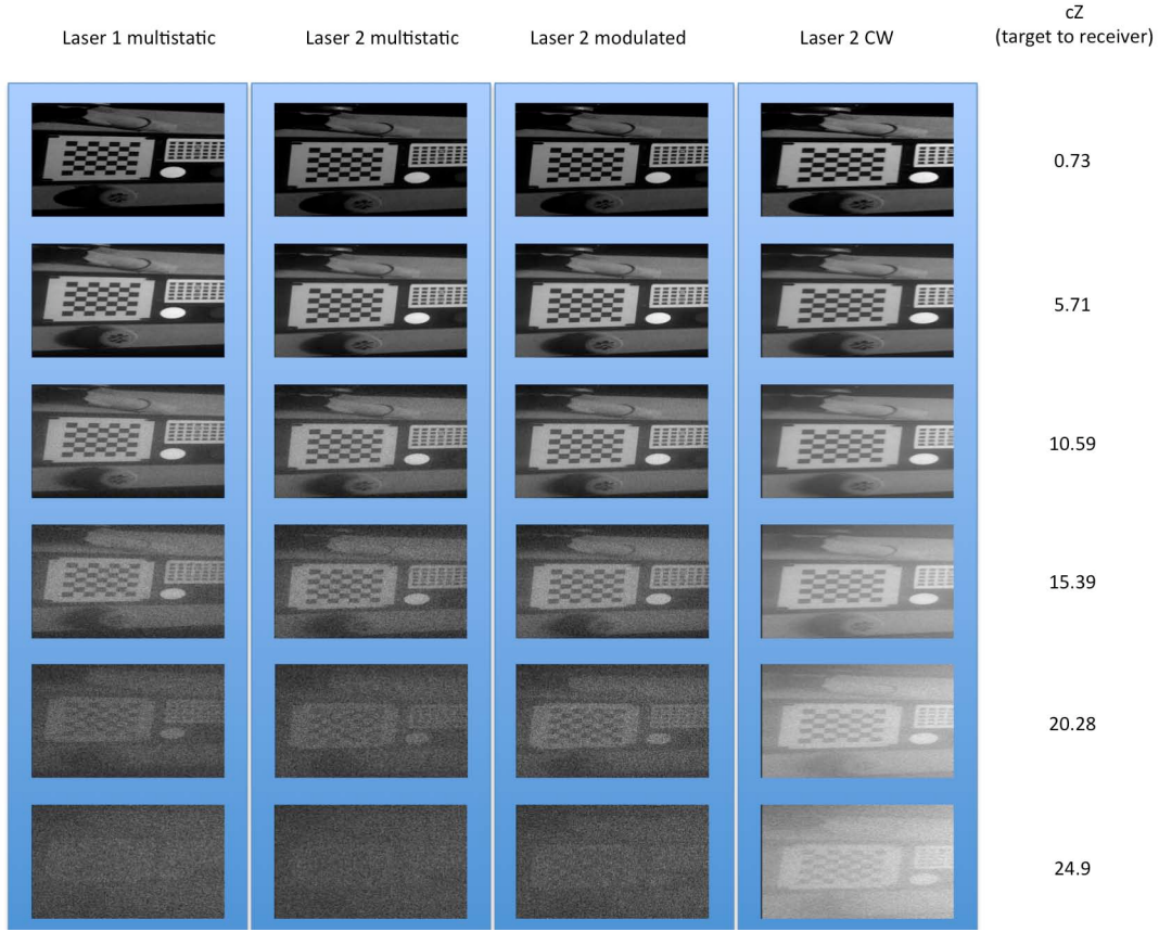
Figure 1: Test tank imaging results for multistatic LLS (columns 1 and 2, 104MHz carrier and 124MHz carrier, respectively), modulated-CW bistatic LLS (column 3, 124MHz carrier) and CW bistatic LLS (column 4). The number of beam attenuation lengths between target and receiver are shown on the right hand side. Average laser power was 35mW for all cases and frame scan period was 2 seconds. The optical receiver was a Hamamatsu 8mm diameter miniature PMT with 50mm diameter f0.83 Lens. The total FOV of the receiver was 9 degrees with flat top response. All images are stretched from min to max. (please note that laser 1 and laser 2 are scanning separate images, albeit with significant overlap)
