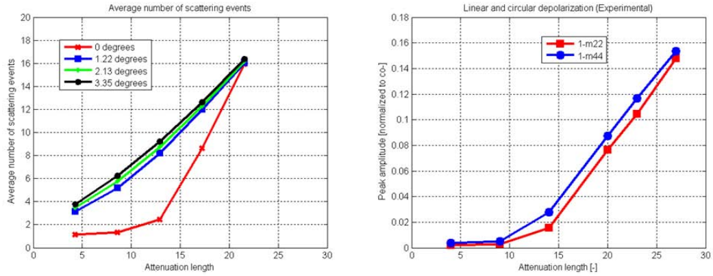
Figure 8: Simulated average number of scattering events (left) and measured Mueller Matrix elements (right) m_{22} and m_{44} at increasing turbidity (magnesium hydroxide).
