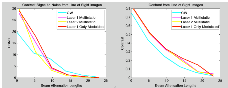
Figure 2: CSNR and contrast image quality metrics for images presented in figure 1.
