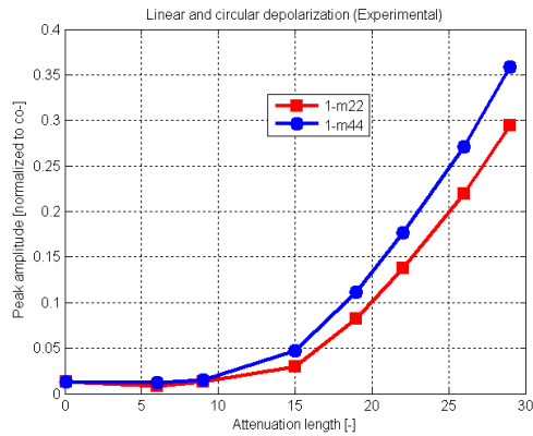
Figure 9: Measured Mueller Matrix elements m_{22} and m_{44} at increasing turbidity (Arizona Test Dust).
