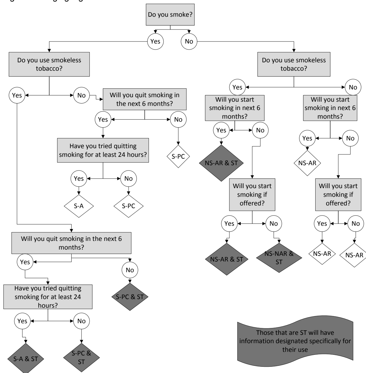
Figure 2. Staging algorithm
