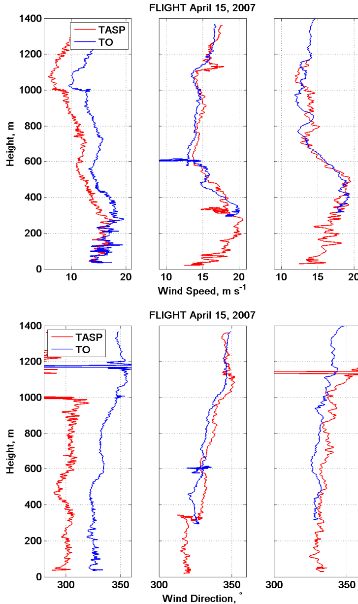
Figure 5: TASP (red) and Twin Otter (blue) profiles of wind speed (top) and direction (bottom) from the 3 soundings ending at 18:35 (left), 18:56 (center) and 20:55 (right) UTC (see Fig. 2). The data were low-pass filtered at 0.25 Hz cutoff frequency for clarity and to reduce the nose wheel wake signature from first sounding data when the TASP was in stowed position.
