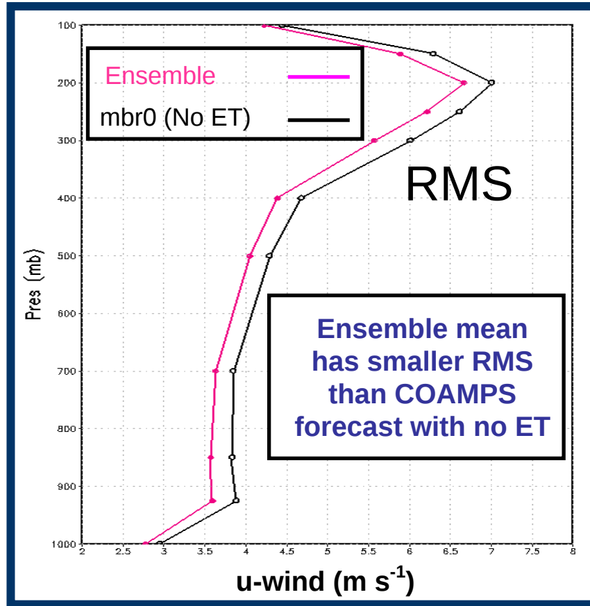
Fig. 3. COAMPS 48-h ensemble forecasts for the 45-km CONUS domain from 25 June to 17 July 2005 of the vertical profile of RMS u-wind ( \text{m s}^{-1} ) of the ensemble mean (magenta) and the control member without ET (black).
