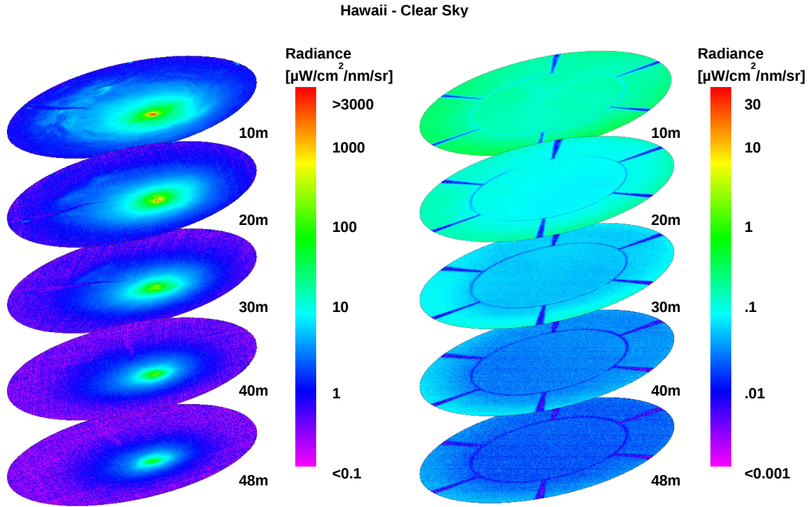
Figure 2: Vertical variation in the downwelling and upwelling radiance distribution in Hawaiian waters. The panel on the left shows the downwelling radiances approximately every 10 meters from the surface to 50 meters. The Sun is clearly evident, as is the Snell cone; the radiance field becomes more diffuse with depth. The panel on the right shows the same, except for the upwelling radiances.
