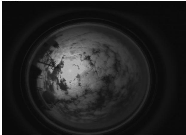
Figure 3: Downwelling sky radiance distribution during the Hawaii experiment. Note patchy cloud distribution and resulting complex radiance field.
