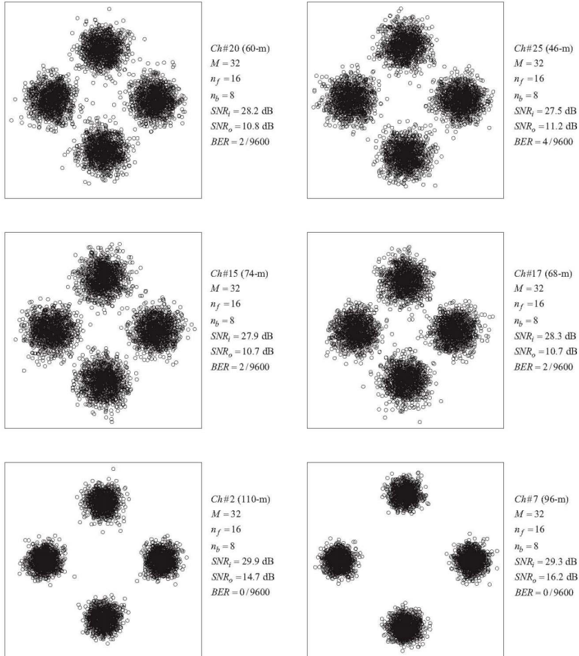
Figure 4. Scatter plots for six users ( N = 6 ) using QPSK: Ch #2 (110 m), Ch #7 (96 m), Ch #15 (74 m), Ch #17 (68 m), Ch #20 (60 m), and Ch #25 (46 m). The aggregate data rate is 6 kbits/s.
