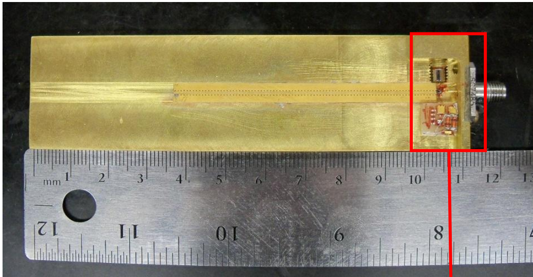
Figure 2 – Spintronics Detector
