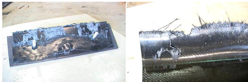
Figure 64. Sample 10 (Failure/Post-Test Damage)
