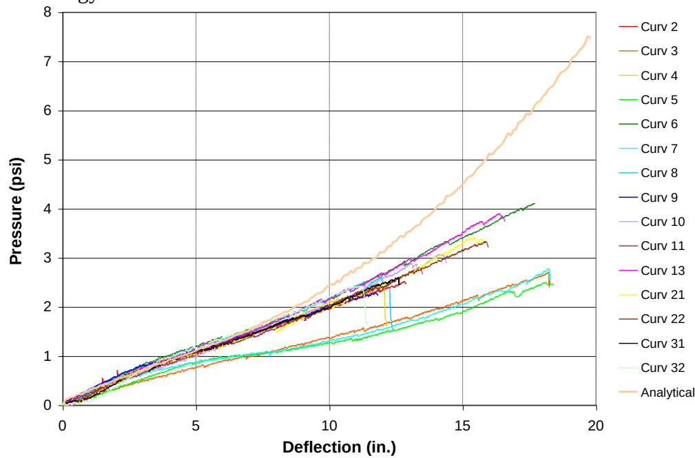
Figure 47. Response Summary of 1-mm Samples
