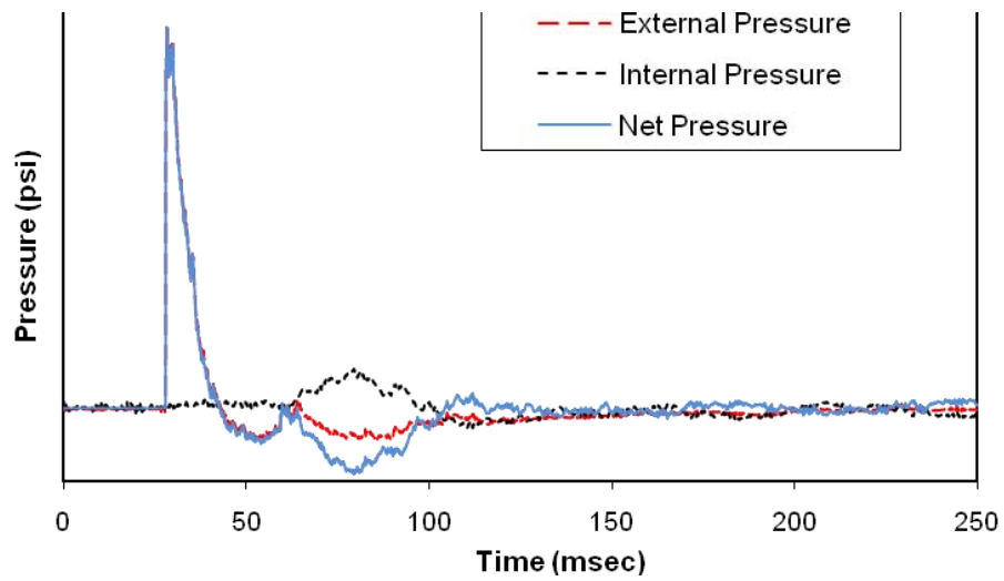
Figure 119. Measured Pressures
