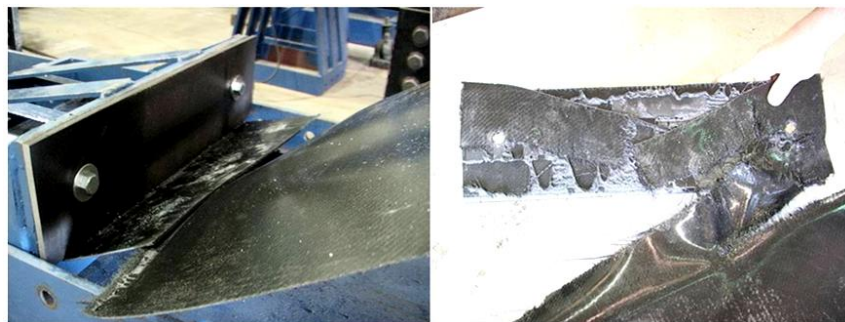
Figure 66. Sample 11 (Failure/Post-Test Damage)
