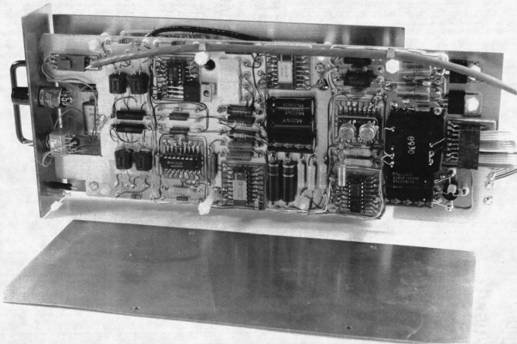
Figure 14. Prototype Conditioner.
