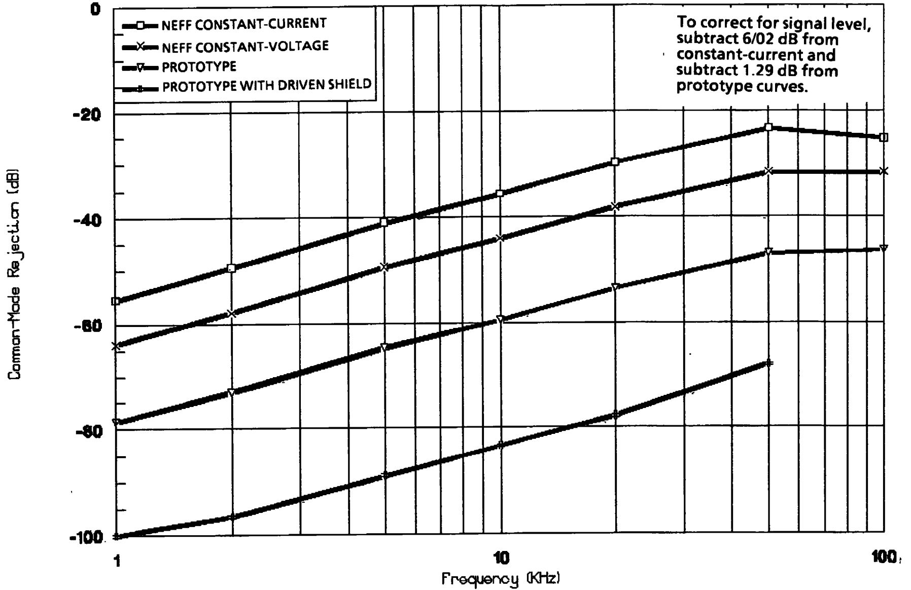
Figure 23. Improvement in Common-Mode Rejection With Driven Shield.
