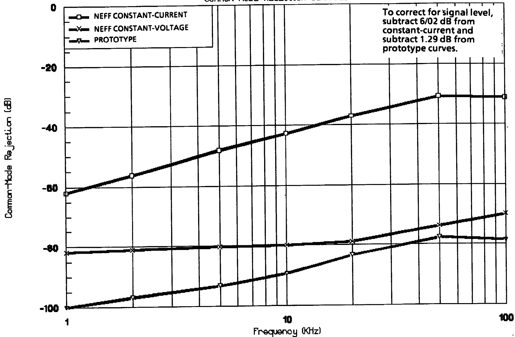
Figure 20. Common-Mode Rejection With Shield Floating at Sensor, Balanced Lead Resistances.
