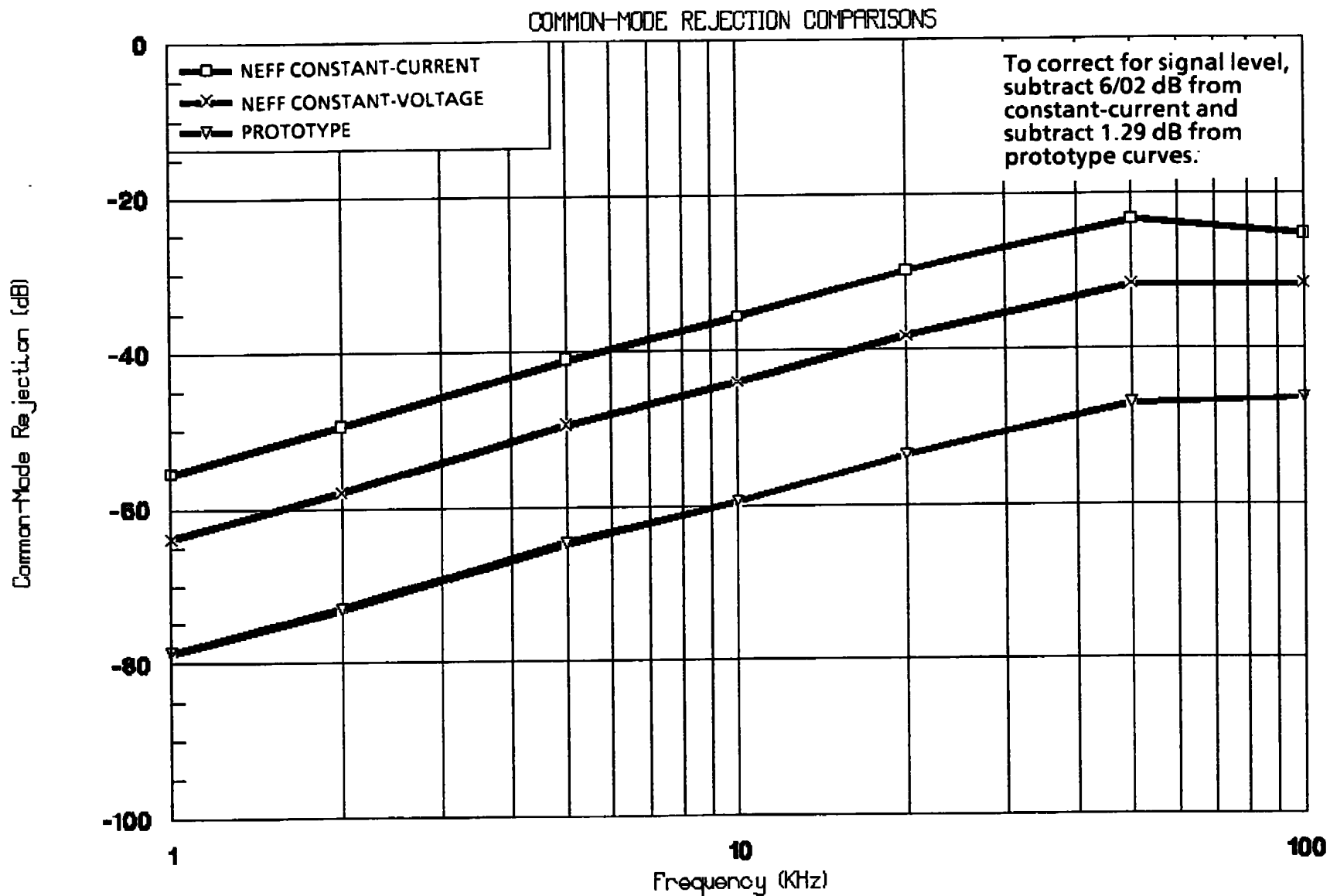
Figure 18. Common-Mode Rejection With Shield Floating at Sensor, Unbalanced Lead Resistances.
