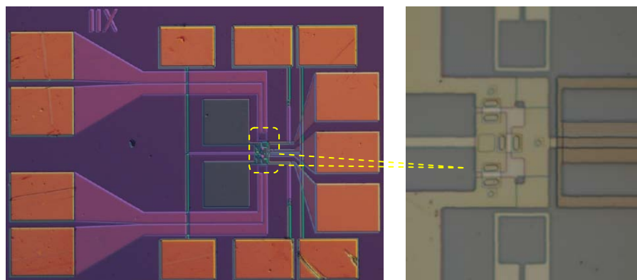
Figure 4. (a) Image of the two cell SQUID circuit with three JJs. The microwave radiations were provided by two microwave sources though two coplanar striplines. (b) The insert showing the two-cell SQUID
