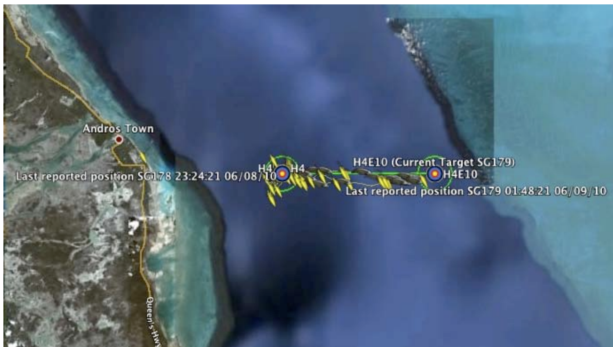
Figure 3. Seaglider™ deployment at AUTECH: 7-11JUN2010, showing sg178 station keeping at H4, and sg179 running east-west transects from H4 to the eastern edge of the AUTECH hydrophone array.
