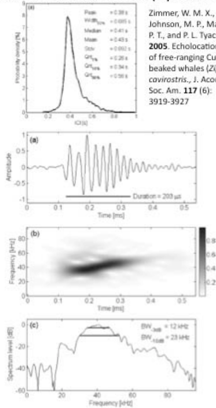
FIG. 2. Sample click of Ziphius click as received by the tag of a conspecific whale. The top panel shows the time series, the middle panel shows the spectrogram (linear spectral scale, Hanning window for FFT of 32 samples, and overlap of 31 samples) and bottom panel shows the relative power spectrum.
