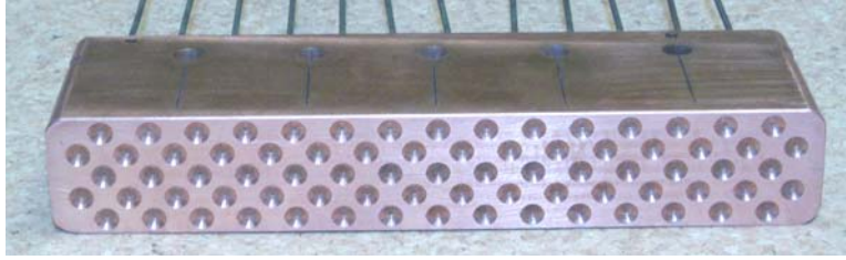
Figure 3 Typical specimen prior to test
