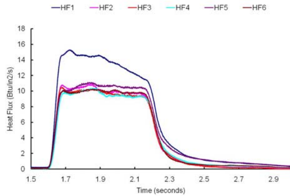
Figure 4 Heat flux traces, CSD pattern #2, sensor #1 exhibits anomalous heat flux due to proximity to leading edge
