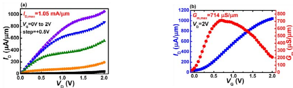
Fig. 1 (a) Drain current ( I_D ) vs. drain bias ( V_D ) of a 1 \mu\text{m} (length) \times 10 \mu\text{m} (width) inversion-channel \text{Al}_2\text{O}_3/\text{GGO}/\text{In}_{0.53}\text{Ga}_{0.47}\text{As} MOSFET. A maximum I_D of 1.05 \text{mA}/\mu\text{m} is measured at gate bias ( V_G ) = 2V and V_D = 2\text{V} ; (b) The transfer characteristics and transconductance ( G_m ) curve of the same device showing a maximum G_m of 714 \mu\text{S}/\mu\text{m} , measured at V_G = 0.7\text{V} and V_D = 2\text{V}
