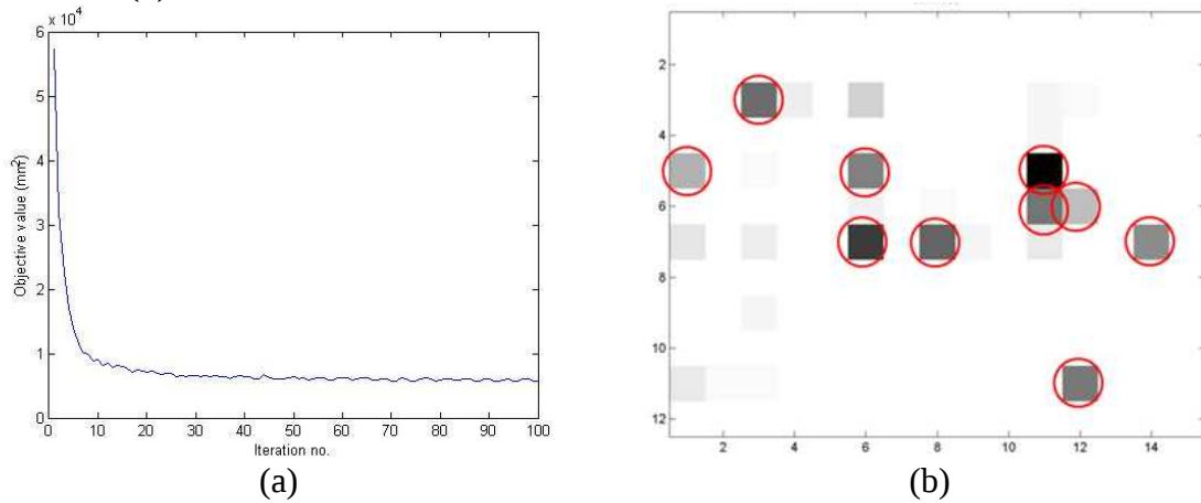
Figure 12. Optimization iteration results (a) and interactive members' final stiffness distribution (b)
