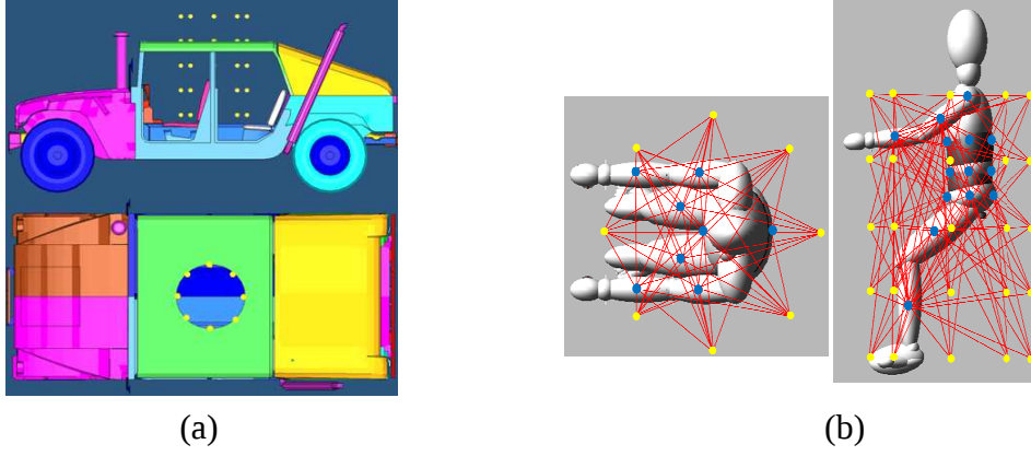
Figure 10 Initial structural universe with connecting points on (a) vehicle and (b) occupant
