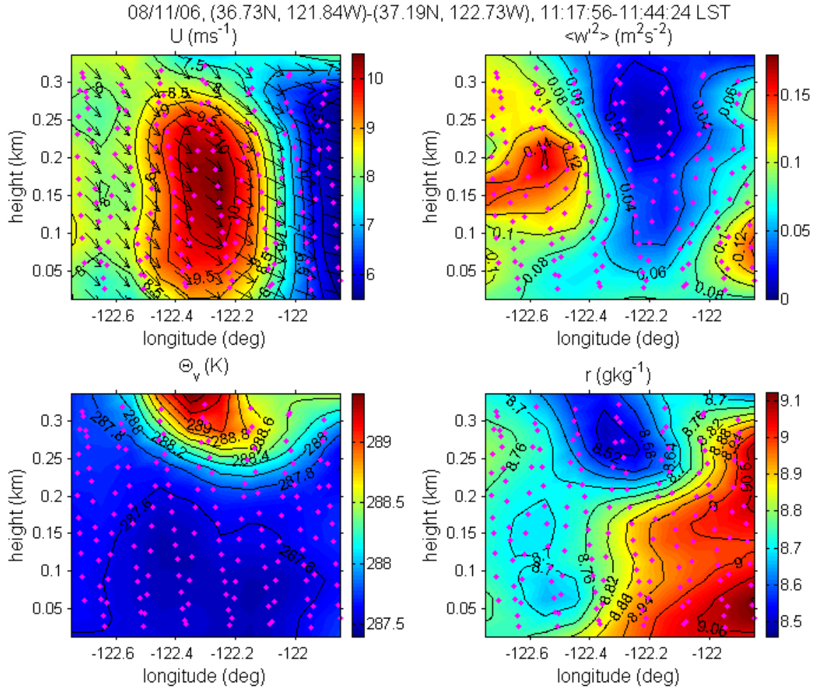
Figure 8: Cross sections of wind speed ( U ), virtual potential temperature ( \Theta_v ), vertical velocity variance ( \langle w'^2 \rangle , 500 m horizontal averaging legs) and water vapor mixing ratio ( r ) using the sawtooth soundings on 8/11/2006 (see Fig. 1). Purple dotted lines denote the flight tracks used to generate the plots.
