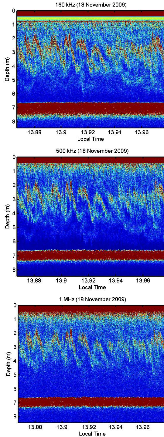
Figure 2. Broadband acoustic backscattering from salinity microstructure in the CT River in November 2009 using the a) 160 kHz BB, b) 500 kHz BB, and c) 1 MHz BB channels of the second-generation WHOI broadband acoustic backscattering system. Kelvin-Helmholtz shear instabilities are apparent in the data. It can be seen that the scattering from the shear instabilities is qualitatively similar at all frequencies.
