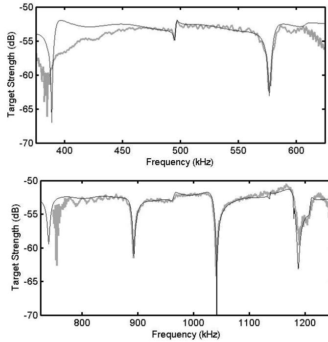
Figure 1. Comparison of the theoretical scattering prediction for an 8.9 mm diameter spherical tungsten carbide standard target, based on the exact modal series solution, to the measured scattering(gray lines) using the second-generation WHOI autonomous broadband acoustic scattering system for the custom-built 500 kHz (upper panel), and 1 MHz (lower panel) almost-octave-bandwidth Airmar broadband transducers.
