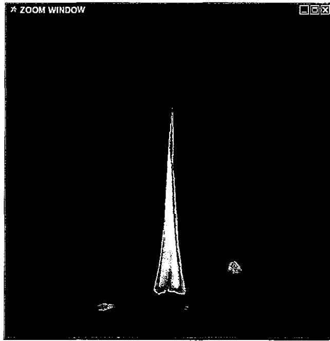
Fig. 5. HIP 40001 and its companion star.
