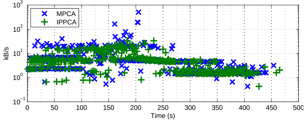
Figure 69: IPPCA vs. MPCA: The communication flow analysis: network flow distribution in time in one specific run for 90 UAAs (bottom).
