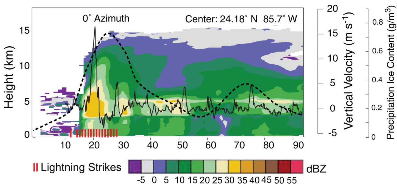
Fig. 10 Vertical reflectivity profile (VRP) composites created by the NOAA P-3 aircraft tail radar during an azimuthal eyewall cross-section flown at 1536 UTC 21 September, with aircraft altitude of 2,600 m and heading of 000°. Overlaid onto the cross-section is flight level vertical velocity measured along the corresponding flight path (heavy solid line), radial lightning strike locations (red bars) during the time of the radial flight, and radial distribution of level 12 (8 – 10 km) TRMM PIC values (dashed line) obtained from the 1540 UTC satellite pass.
