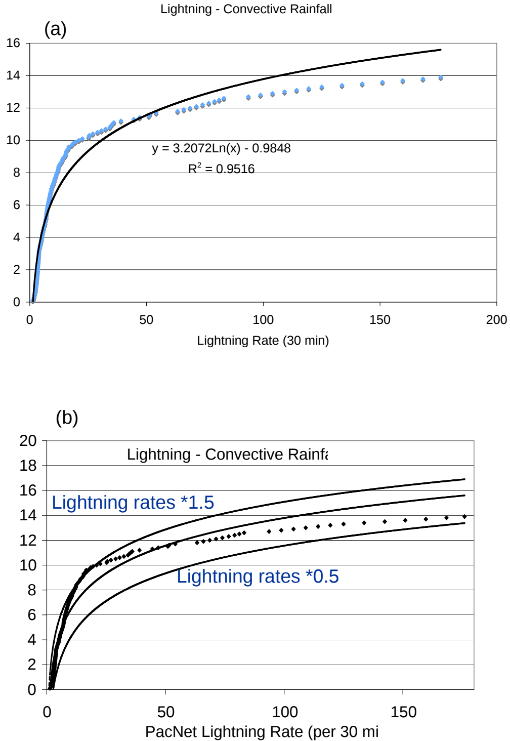
Fig. 3 (a) Relationship of PacNet lightning rate and convective rainfall rate derived from TRMM TMI data based on the cumulative probability matching method. (b) as in (a) with lines for lightning rate multiplied by factors of 1.5 and 0.5, respectively.
