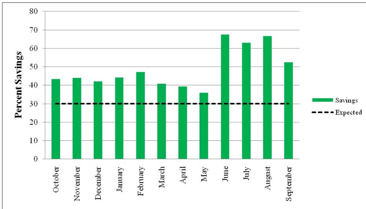
Figure 40 – NFESC/NAVSEA Electricity Consumption Percent Savings
