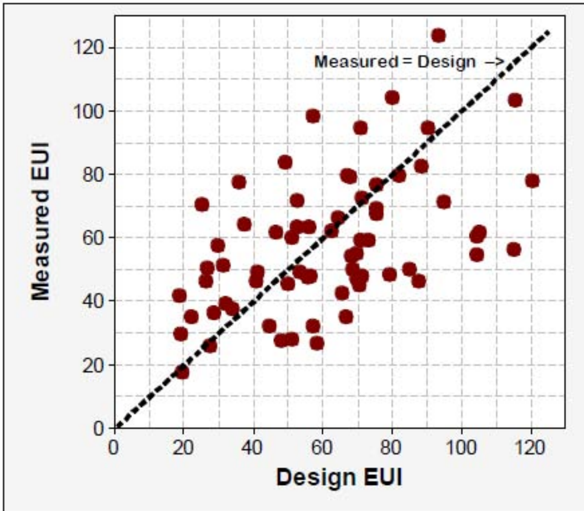
Figure 4 – Measured versus Design EUIs (Turner and Frankel 2008)
