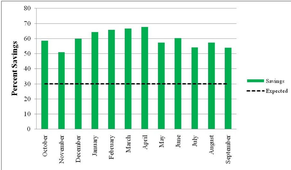
Figure 16 – Airborne Mine/Aircraft Hangar Electricity Consumption Percent Savings
