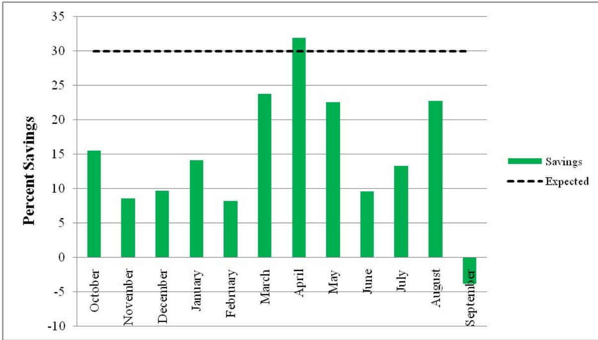
Figure 44 – PWDs Electricity Consumption Percent Savings
