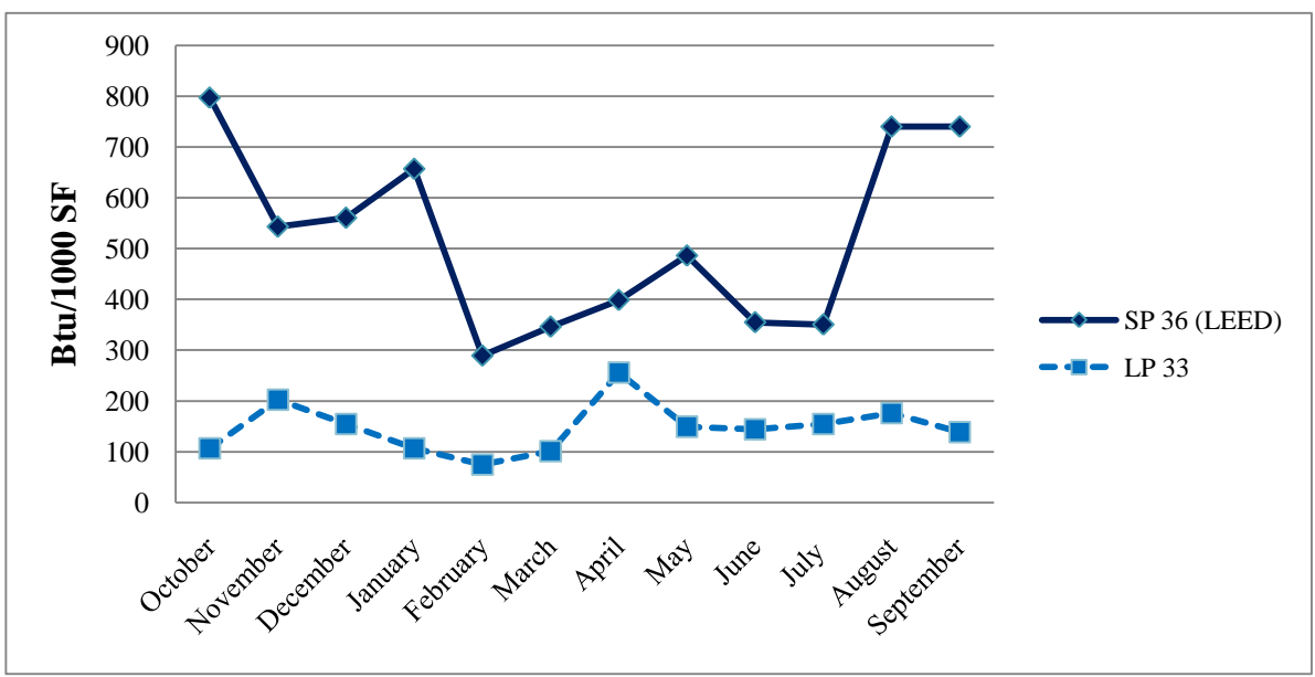
Figure 19 – Aircraft Hangars Monthly Water Consumption Data (Btu/1000 SF)
