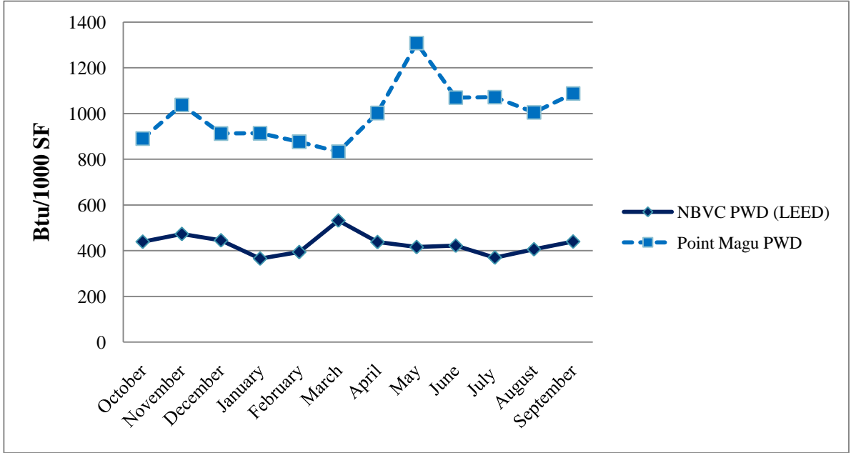
Figure 43 – PWDs Monthly Water Consumption Data (Btu/1000 SF)
