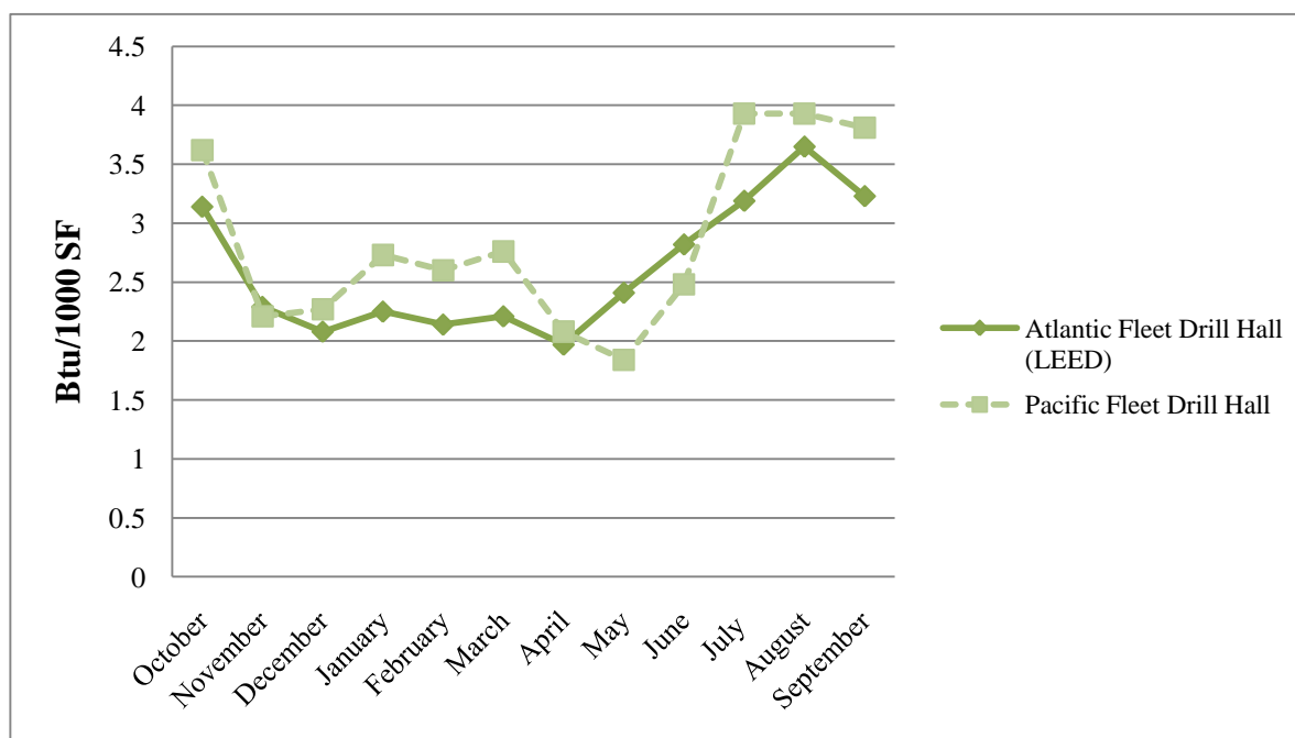
Figure 10 – Drill Halls Monthly Electricity Consumption Data (Btu/1000 SF)
