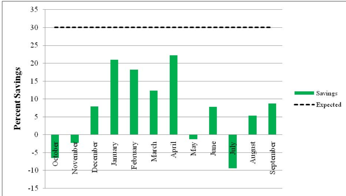
Figure 20 – Aircraft Hangars Electricity Consumption Percent Savings
