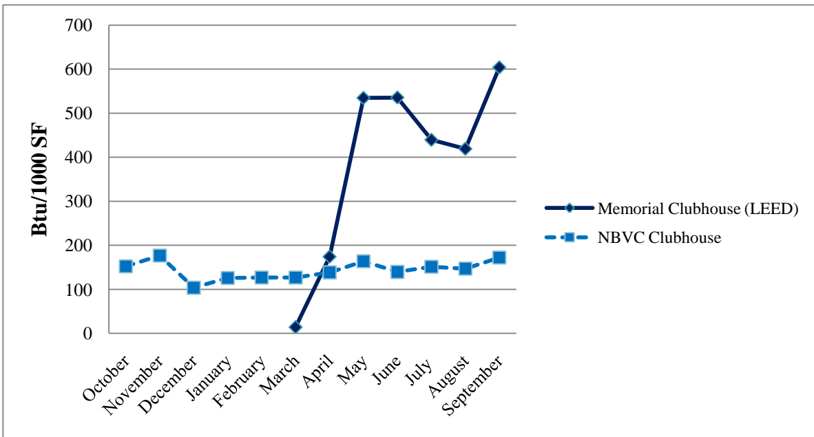
Figure 35 – Golf Course Clubhouses Monthly Water Consumption Data (Btu/1000 SF)
