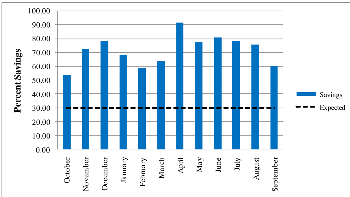
Figure 17 – Airborne Mine/Aircraft Hangar Water Consumption Percent Savings
