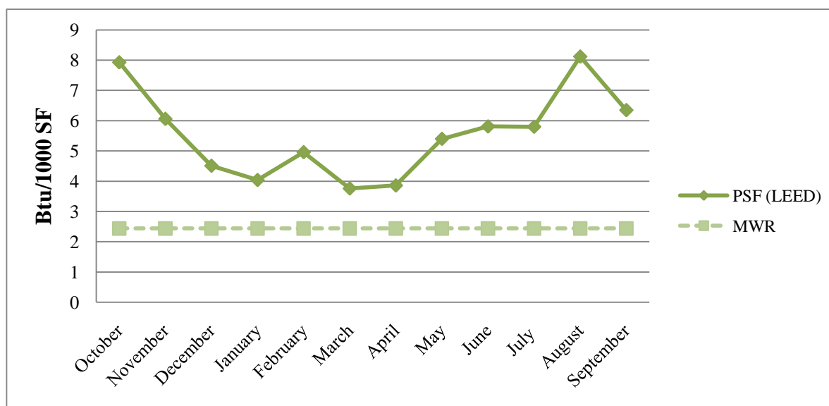
Figure 24 – PSF/MWR Monthly Electricity Consumption Data (Btu/1000 SF)
