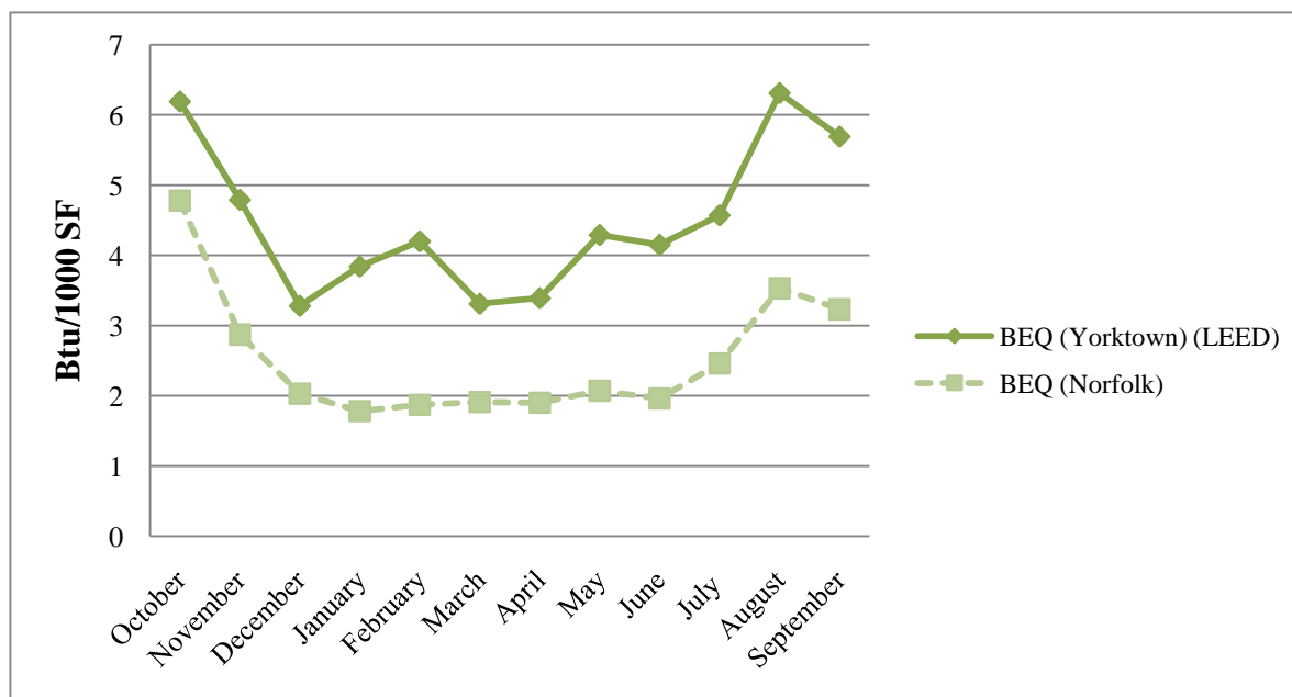
Figure 22 – BEQs Monthly Electricity Consumption Data (Btu/1000 SF)
