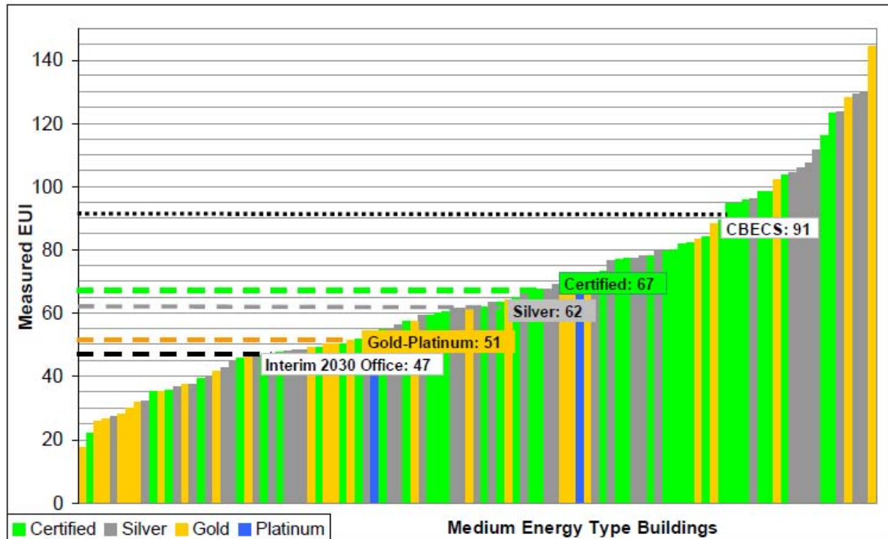
Figure 2 – EUI (kBtu/sf) Distribution (Turner and Frankel 2008)
