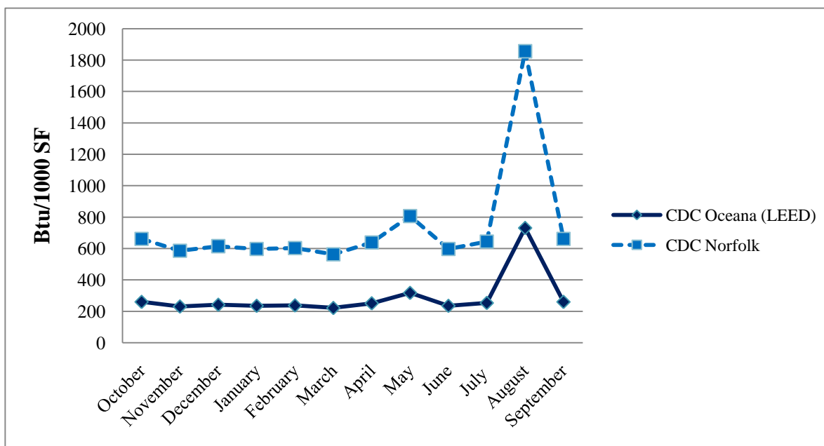
Figure 47 – CDCs Monthly Water Consumption Data (Btu/1000 SF)
