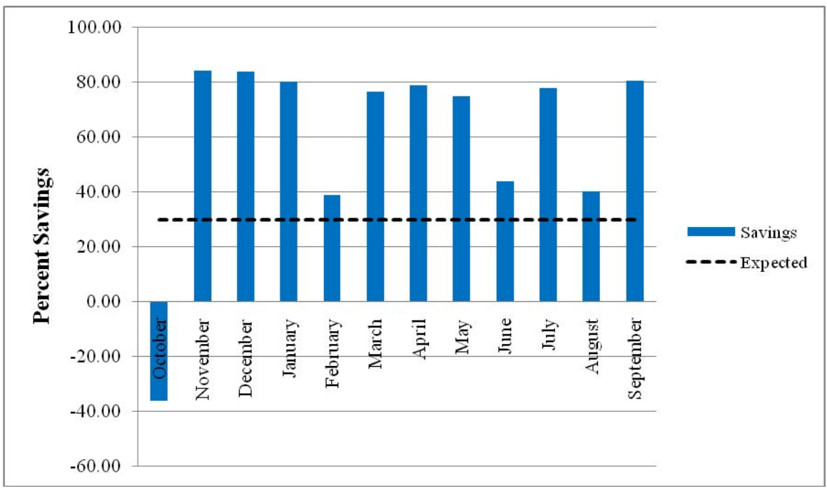
Figure 13 – Drill Halls Water Consumption Percent Savings
