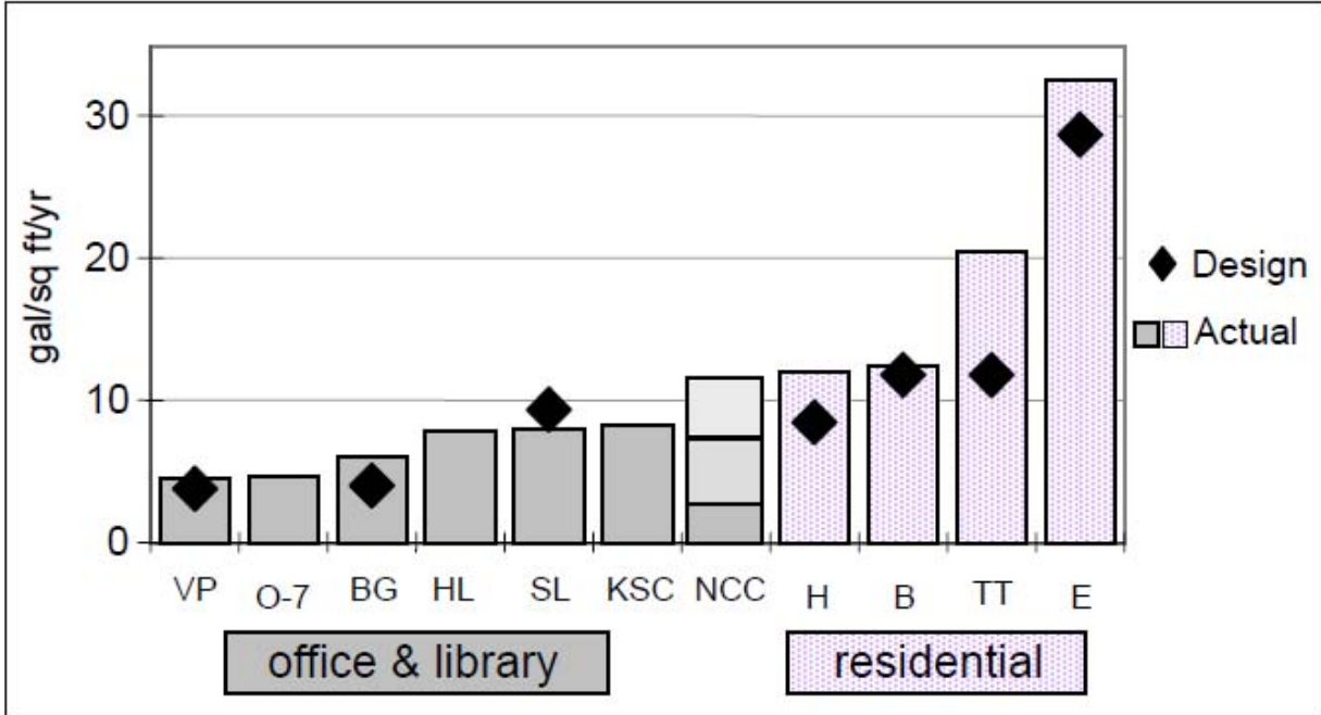
Figure 7 – Actual and Design Water Use per Square Foot (Turner 2006)
