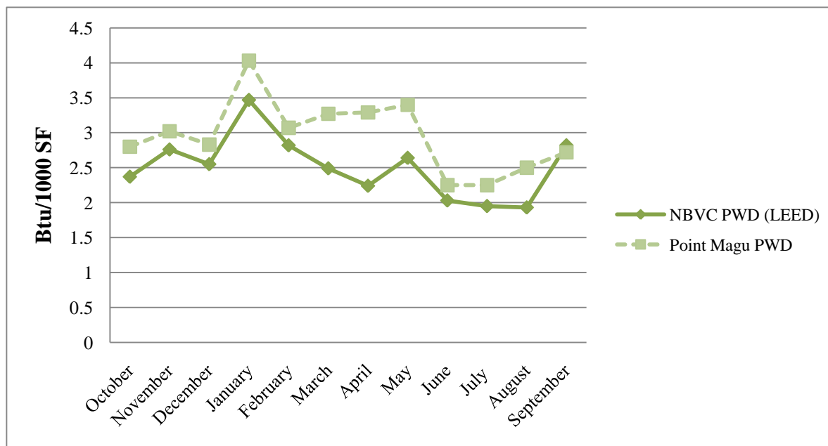
Figure 42 – PWDs Monthly Electricity Consumption Data (Btu/1000 SF)
