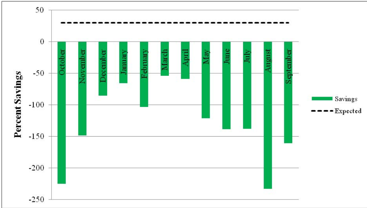
Figure 26 – PSF/MWR Electricity Consumption Percent Savings
