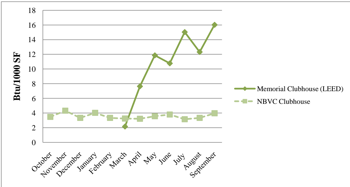
Figure 34 – Golf Course Clubhouses Monthly Electricity Consumption Data (Btu/1000 SF)
