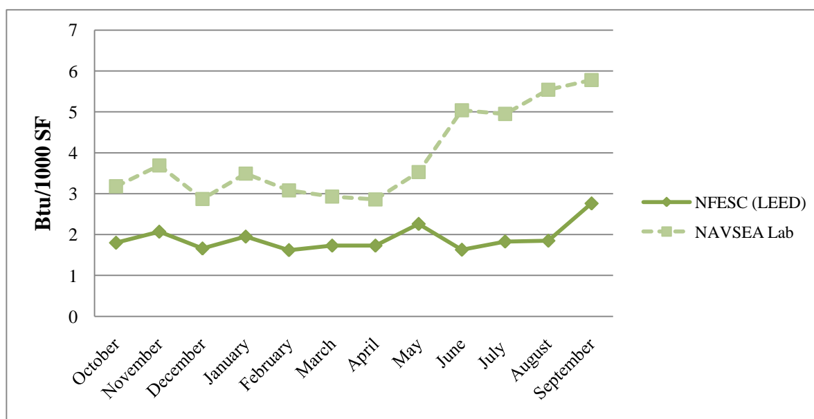
Figure 38 – NFESC/NAVSEA Monthly Electricity Consumption Data (Btu/1000 SF)
