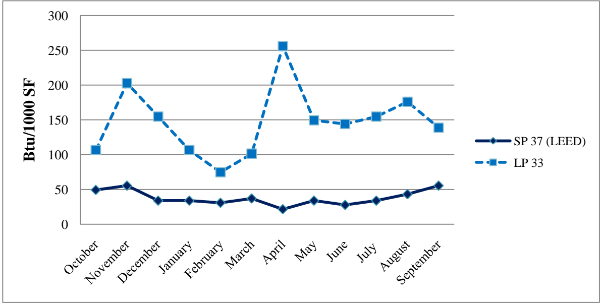
Figure 15 – Airborne Mine/Aircraft Hangar Monthly Water Consumption Data (Btu/1000 SF)
