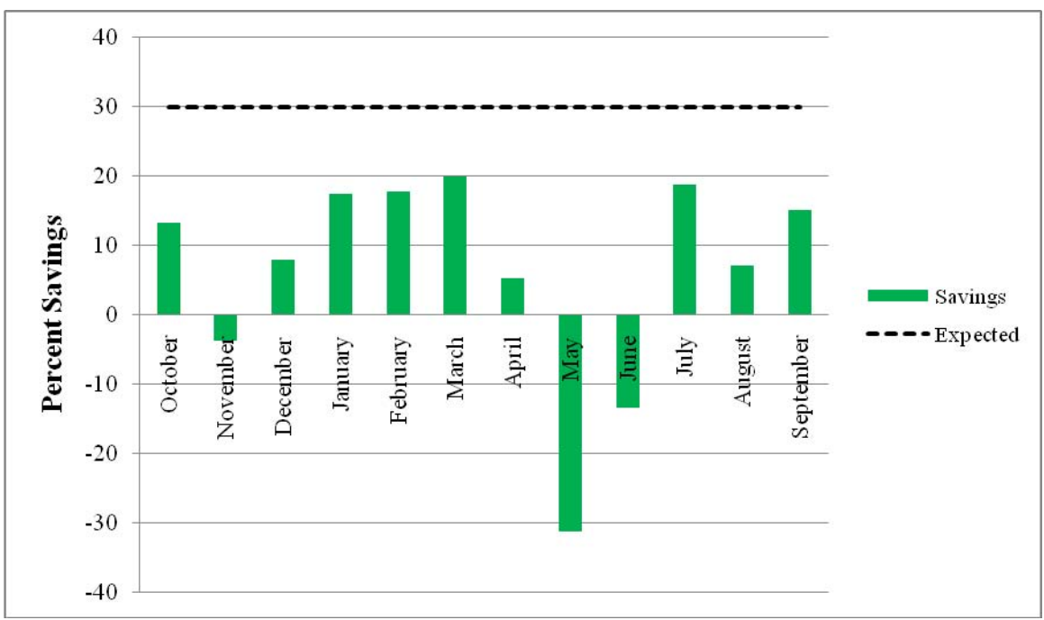
Figure 12 – Drill Halls Electricity Consumption Percent Savings
