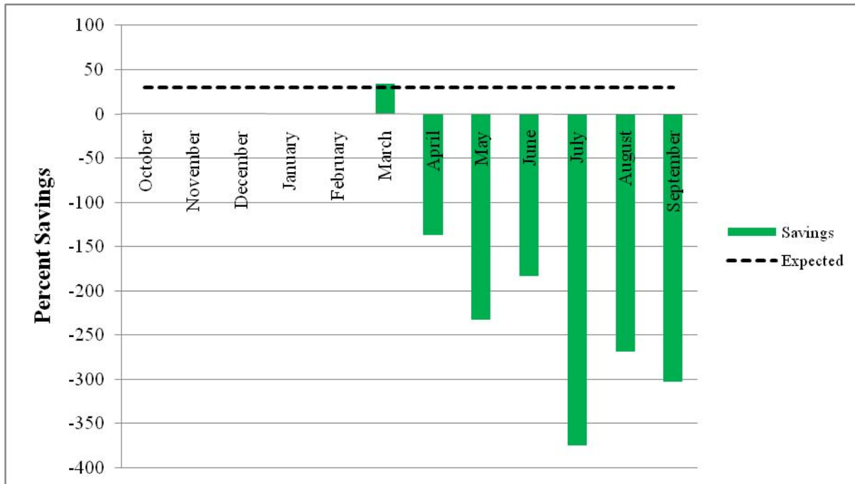
Figure 36 – Golf Course Clubhouses Electricity Consumption Percent Savings
