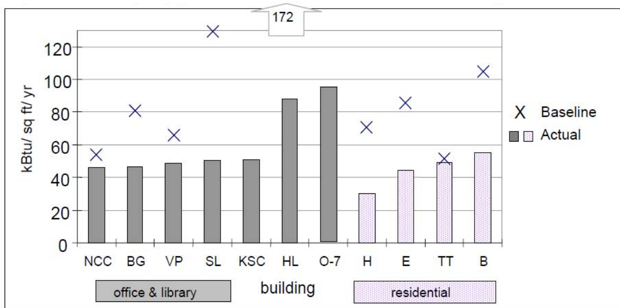
Figure 6 – Actual and Baseline Energy Use Intensities (Turner 2006)
