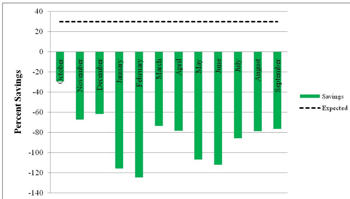
Figure 23 – BEQs Electricity Consumption Percent Savings
