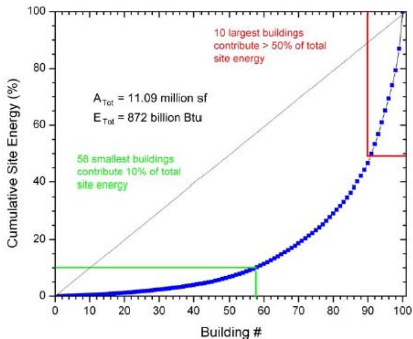
Figure 5 - The cumulative contribution to the total site energy of the 100 medium energy LEED buildings sorted by building site energy (Scofield 2009)
