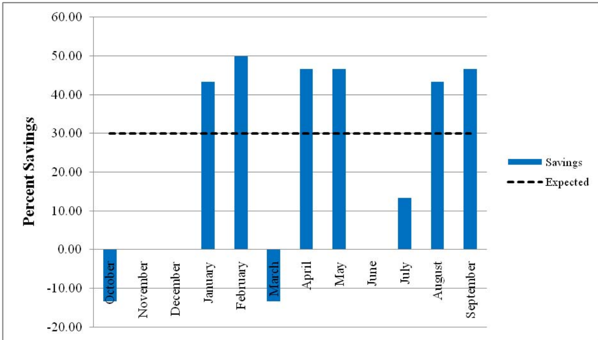
Figure 27 – PSF/MWR Water Consumption Percent Savings
