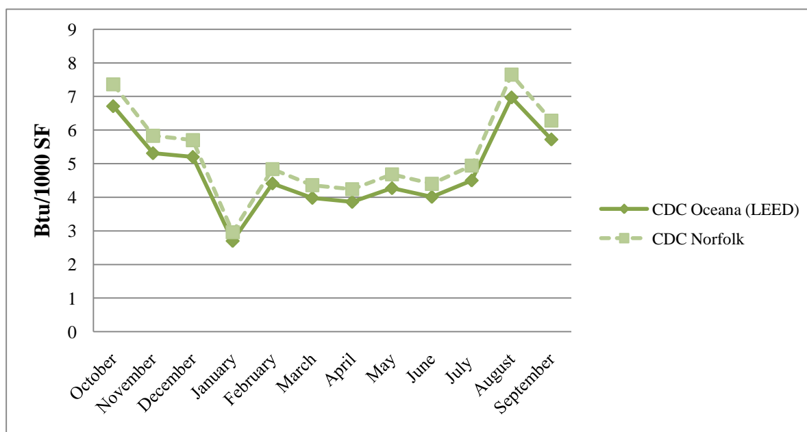
Figure 46 – CDCs Monthly Electricity Consumption Data (Btu/1000 SF)
