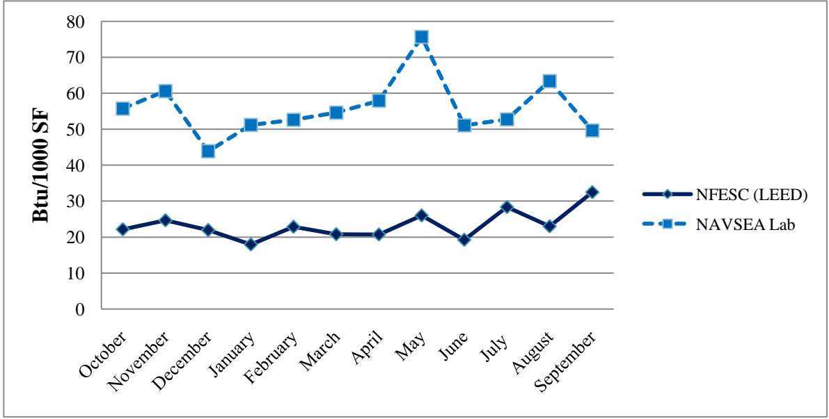
Figure 39 – NFESC/NAVSEA Monthly Water Consumption Data (Btu/1000 SF)
