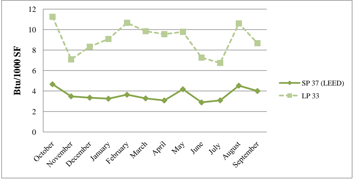
Figure 14 – Airborne Mine/Aircraft Hangar Monthly Electricity Consumption Data (Btu/1000 SF)
