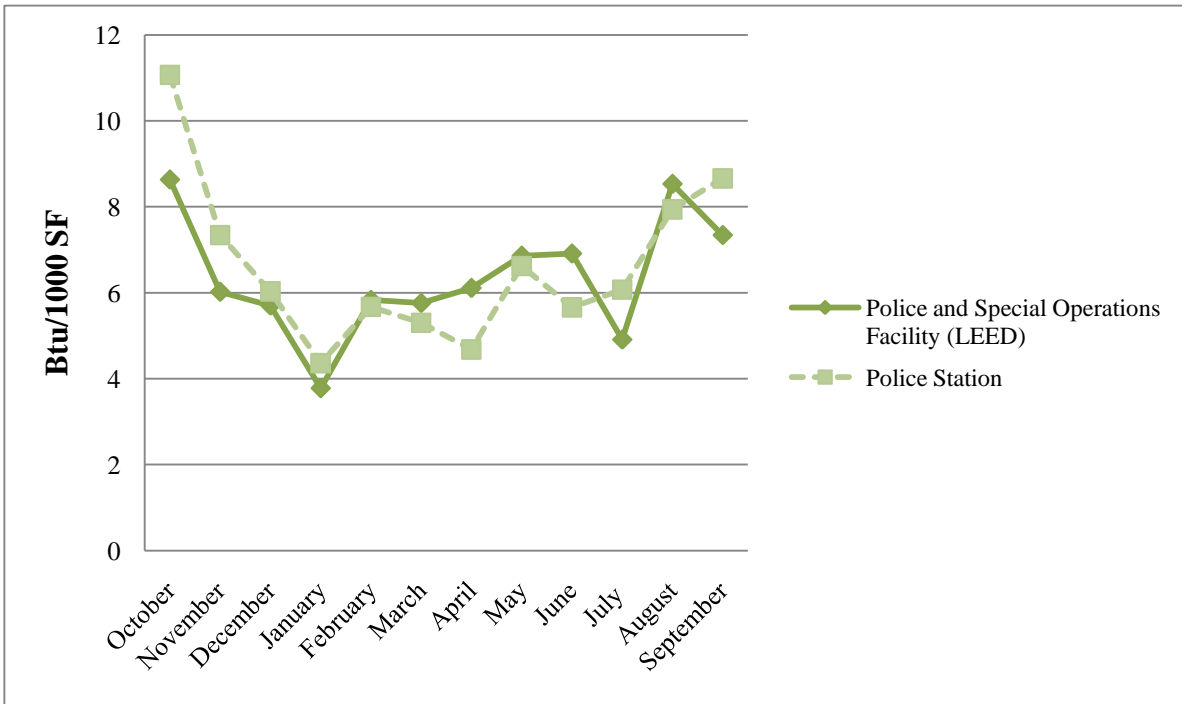
Figure 28 – Police Stations Monthly Electricity Consumption Data (Btu/1000 SF)
