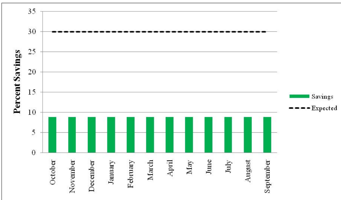
Figure 48 – CDCs Electricity Consumption Percent Savings
