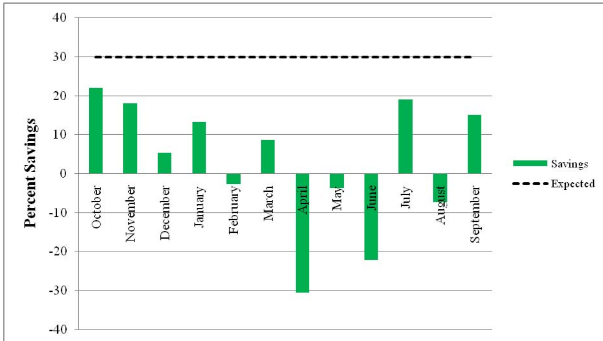
Figure 30 – Police Stations Electricity Consumption Percent Savings
