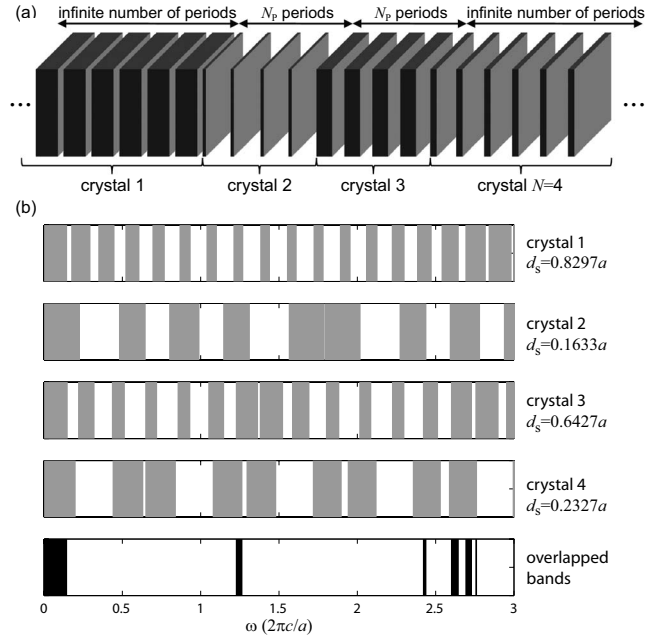
FIG. 1. (a) A photonic crystal heterostructure with four crystals. Each crystal has alternate silicon and vacuum layers, and a period a . The top two crystals at either ends are assumed to be infinite. (b) In the top four panels, gray regions correspond to frequency ranges where the corresponding crystal, assumed to be infinite, has a propagating state along the normal incident direction. White regions are the band gaps. d_s is the thickness of the silicon layers. In the bottom panel, the black regions represent frequency ranges where there are photonic bands in all crystals.
