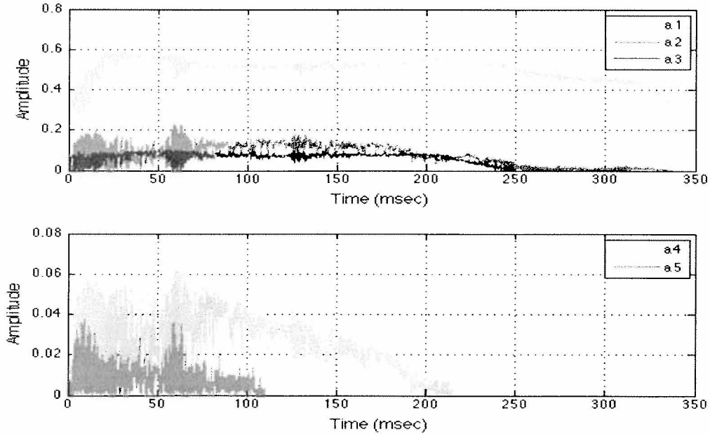
Figure 4-5: Estimated amplitude contours for Whistle 1 in Fig. 4-1
