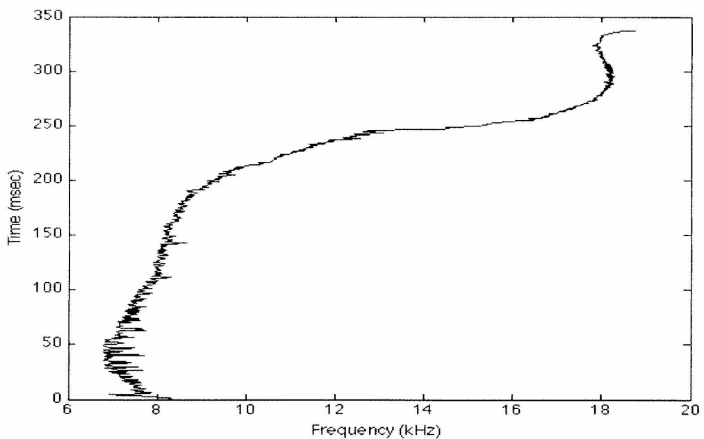
Figure 4-4: Fundamental frequency contour of Whistle 1 in Fig. 4-1
