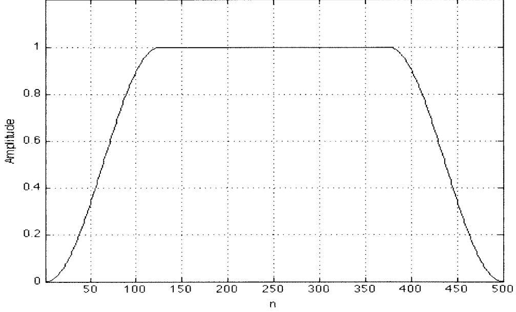
Figure 3-7: Tukey window with \alpha = 0.5
