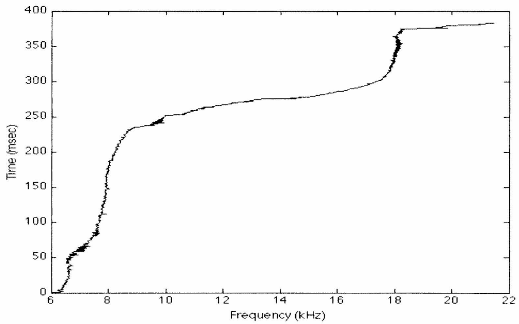
Figure 4-9: Fundamental frequency contour of Whistle 2 in Fig. 4-1
