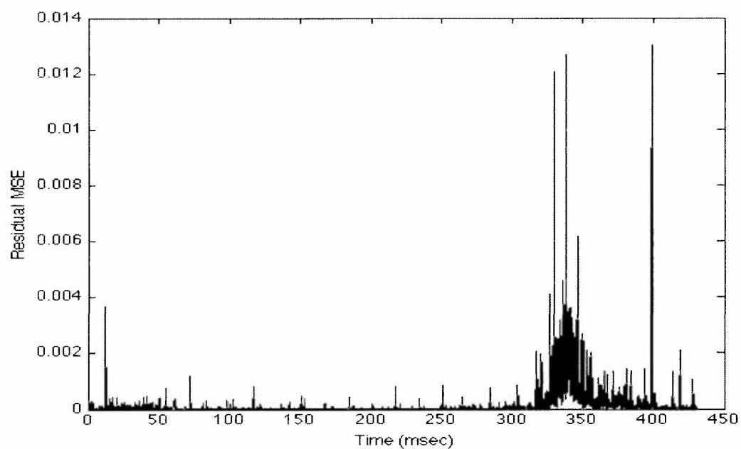
Figure 4-14: Residual MSE for Whistle 3 in Fig. 4-1
