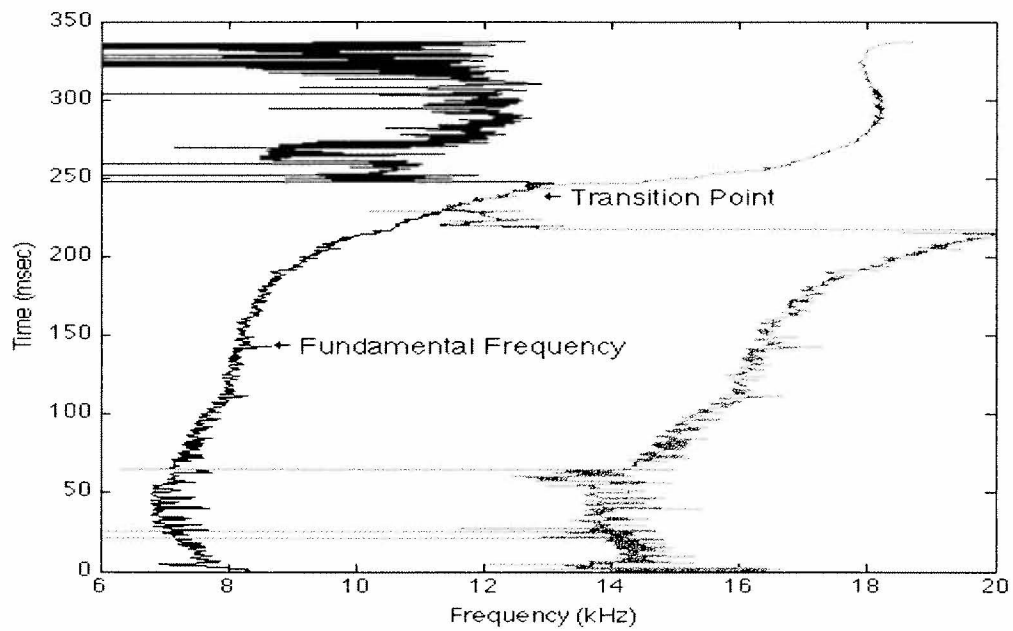
Figure 4-3: Fundamental frequency estimation of Whistle 1 in Fig. 4-1 using overlapping bandpass filters
