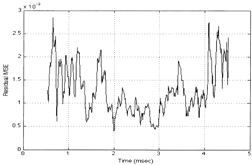
Figure 3-11: Residual MSE for double harmonic linear chirp (SNR = 25 dB)
