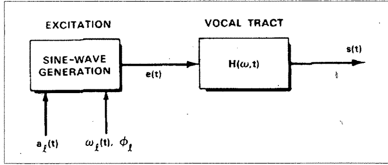
Figure 1-1: Quatieri and McAulay's speech production model [53]
