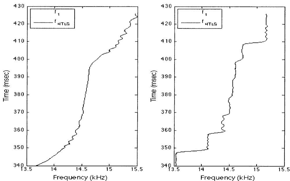
Figure 5-5: Frequency estimation performance for unmodified (left) and watermarked (right) whistle contours received at reference hydrophone
