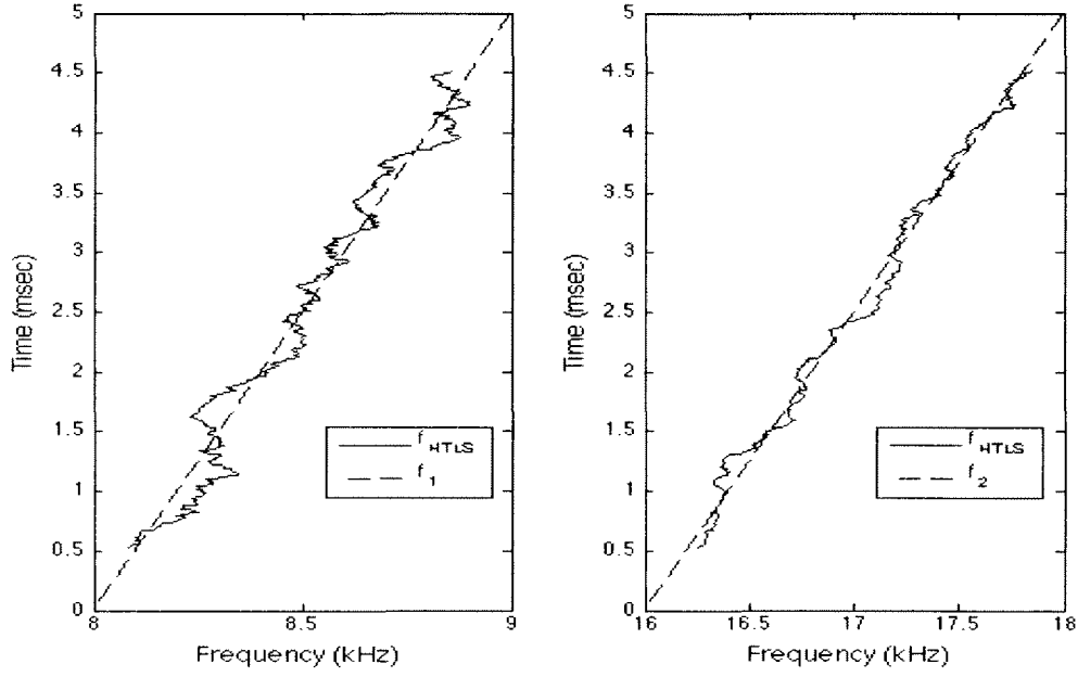
Figure 3-2: HTLS frequency tracking performance for a linear chirp with two harmonics (SNR = 5 dB)
