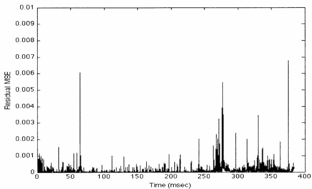
Figure 4-13: Residual MSE for Whistle 2 in Fig. 4-1
