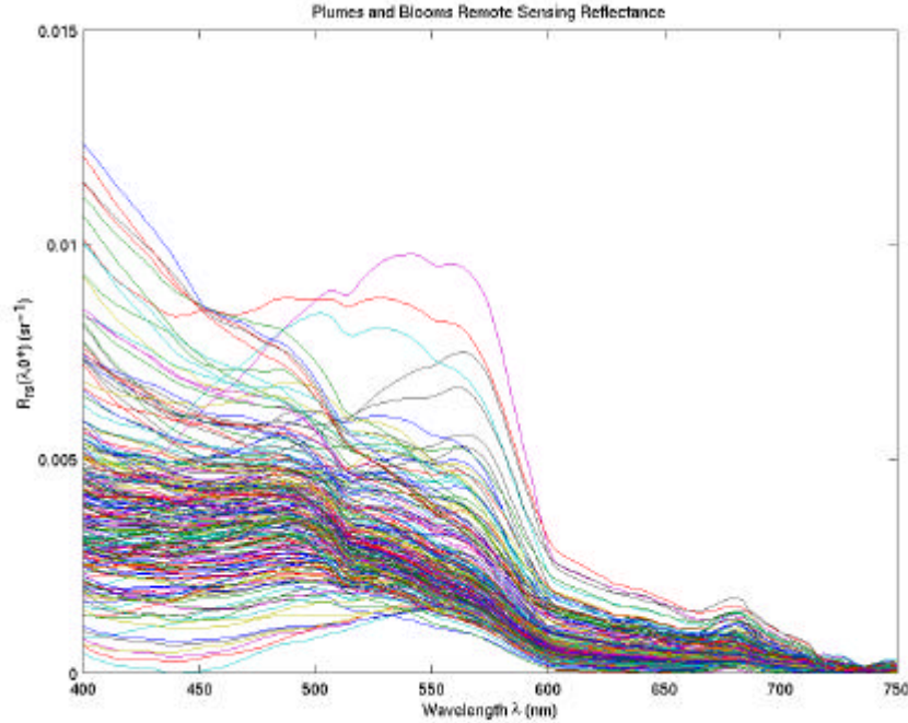
Figure 2: Remote sensing reflectance spectra, R_{rs}^+(l) , taken from the PnB observational program. All observations are shown which were taken between August 1996 and October 1998. The above-water, hand-held spectrometer technique is used to make the present measurements of R_{rs}^+(l) . Contemporaneous determinations of R_{rs}^+(l) are also made using the profiling spectroradiometer and tethered buoy methods (Toole et al. 1998).
